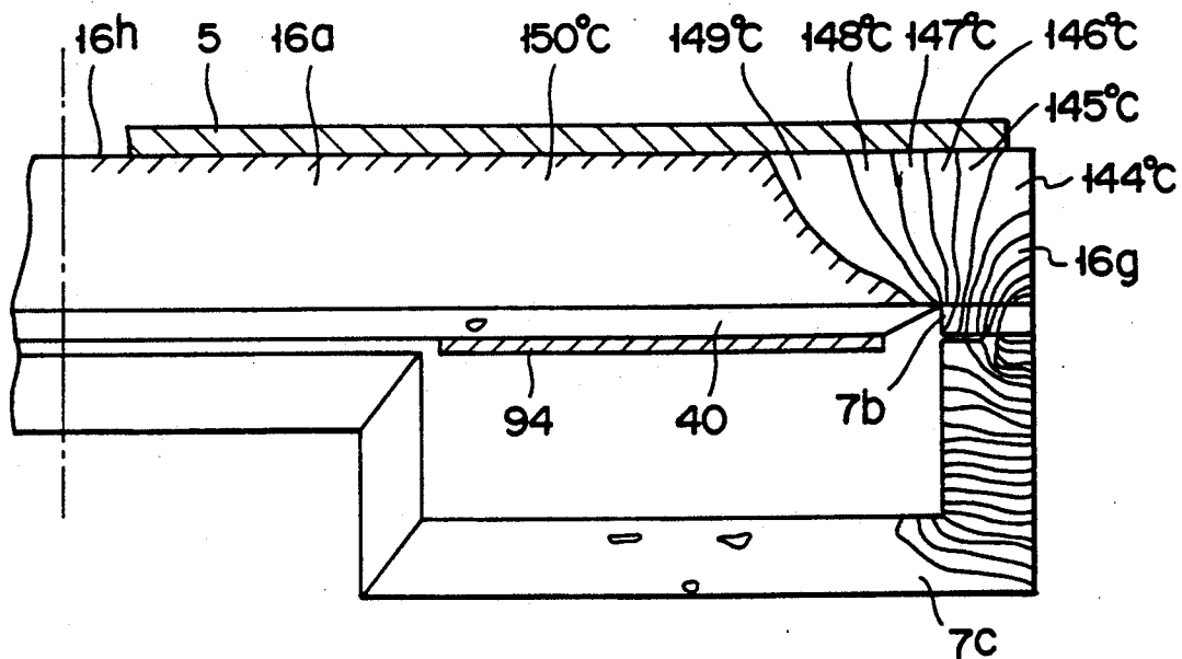
PRIOR ART FIG. 20
