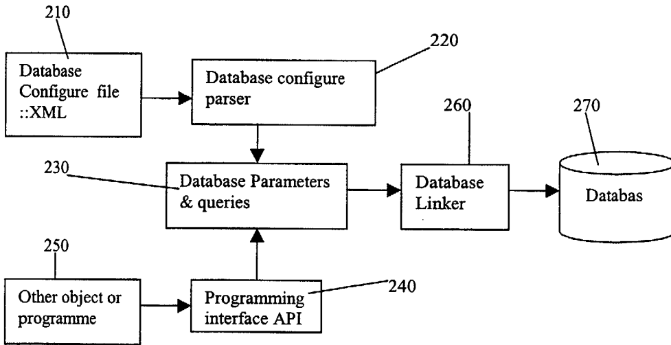
FIG. 2 illustrates database connection and data retrieve module
