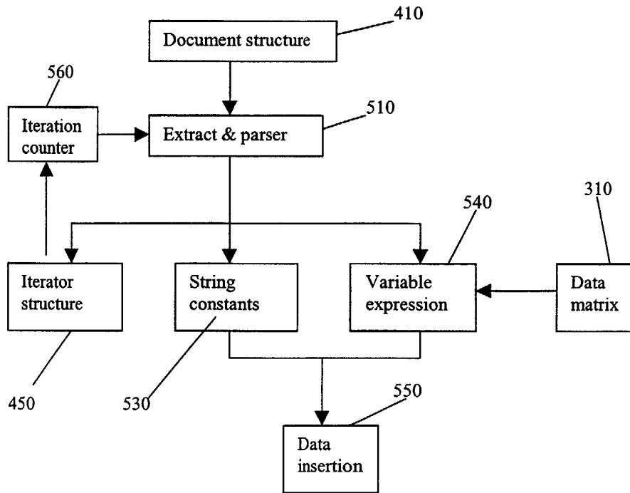
FIG. 5 illustrates the procedure of data insertion
