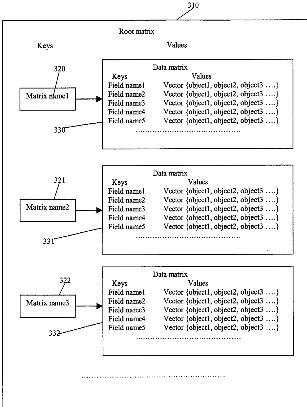
FIG. 3 illustrates the data structure model
