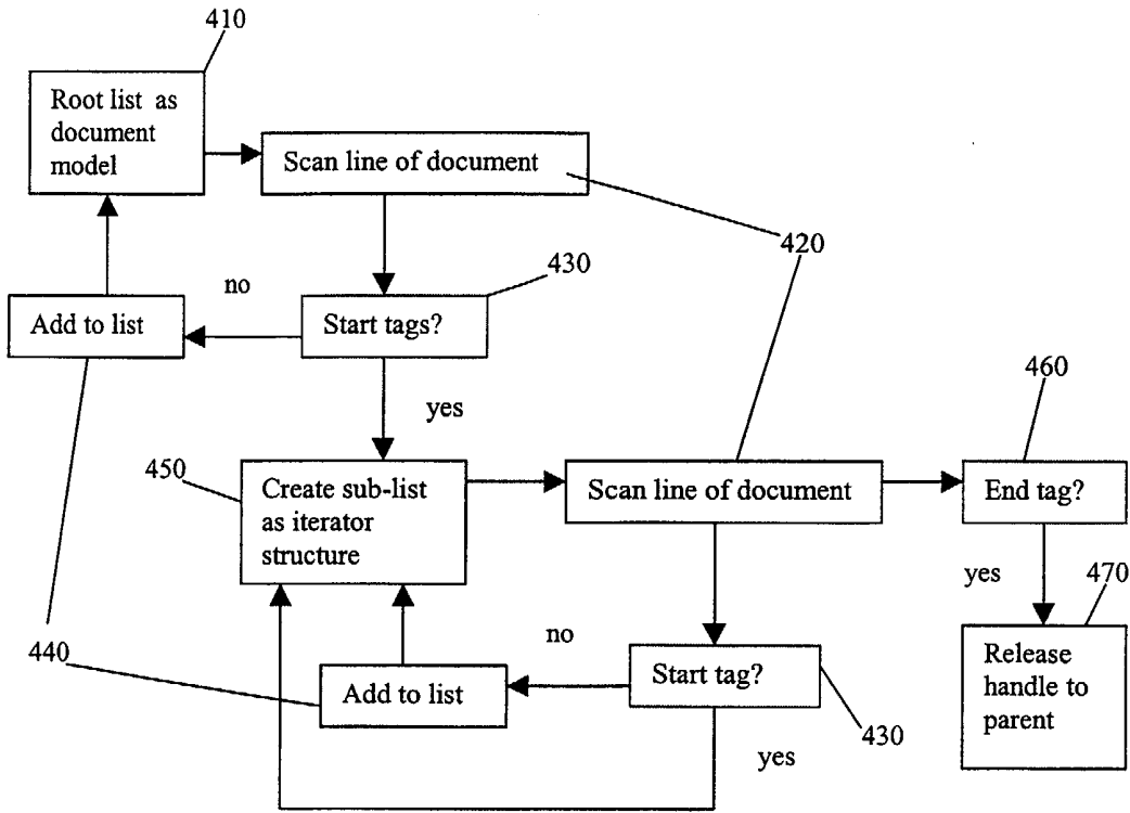
FIG. 4 illustrates the creation of document model
