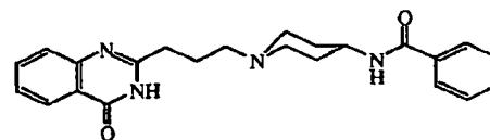
Compound 12
