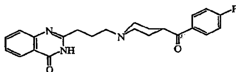
Compound 14
