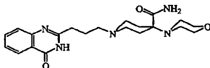
Compound 11
