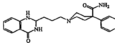
Compound 5
