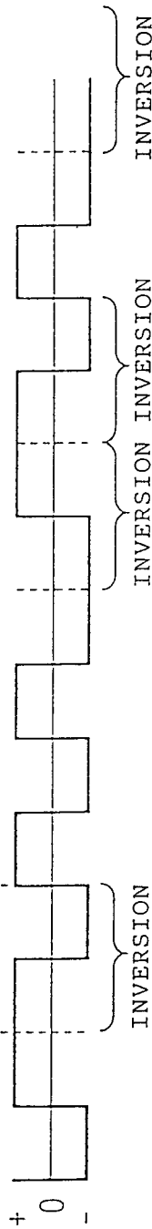
FIG. 16C MODULATING WAVE (DIFFERENTIAL CONVERSION)
