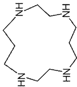
1,4,8,11- tetraazacyclotetradecane
