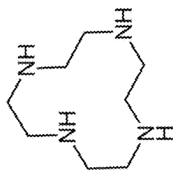
1,4,7,10- tetraazacyclododecane
