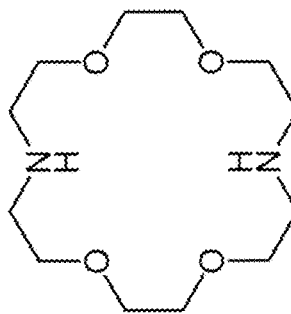
1,4,10,13-tetraoxa-7,16- diazacyclooctadecane
