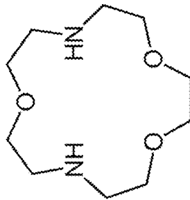
1,4,10-trioxa-7,13- diazacyclopentadecane
