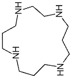
1,4,8,12- tetraazacyclopentadecane
