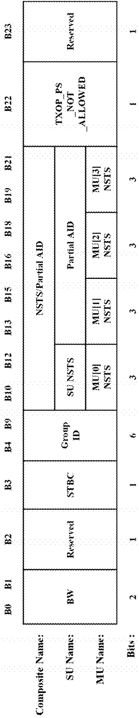
VHT-SIG-A1 Structure
