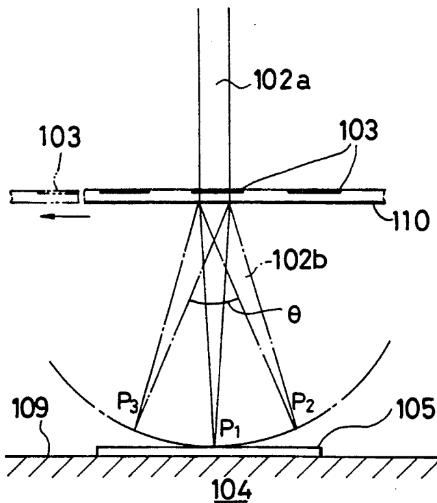
FIG. 2 PRIOR ART
