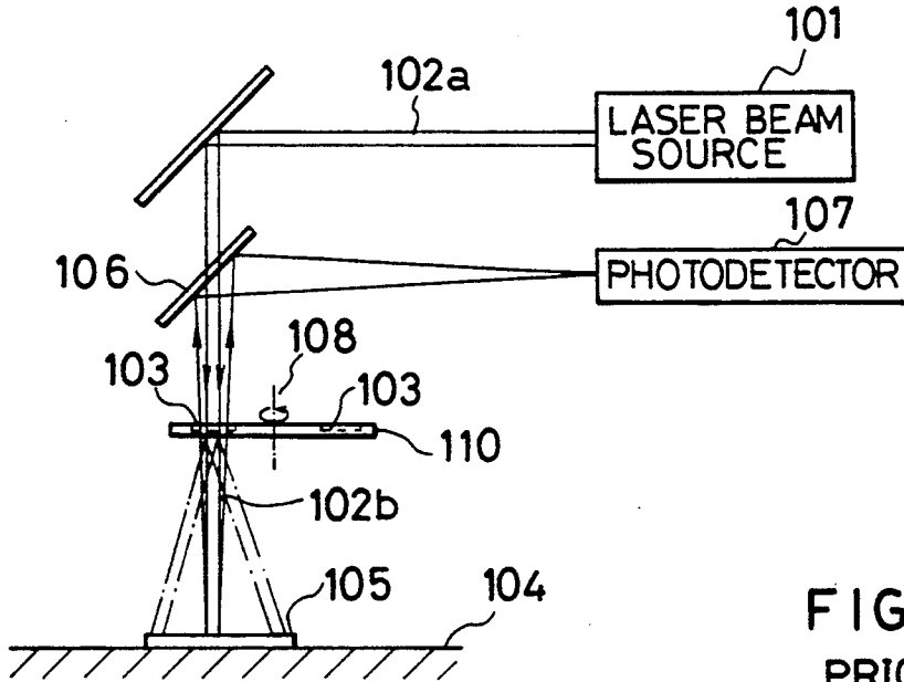
PRIOR ART
