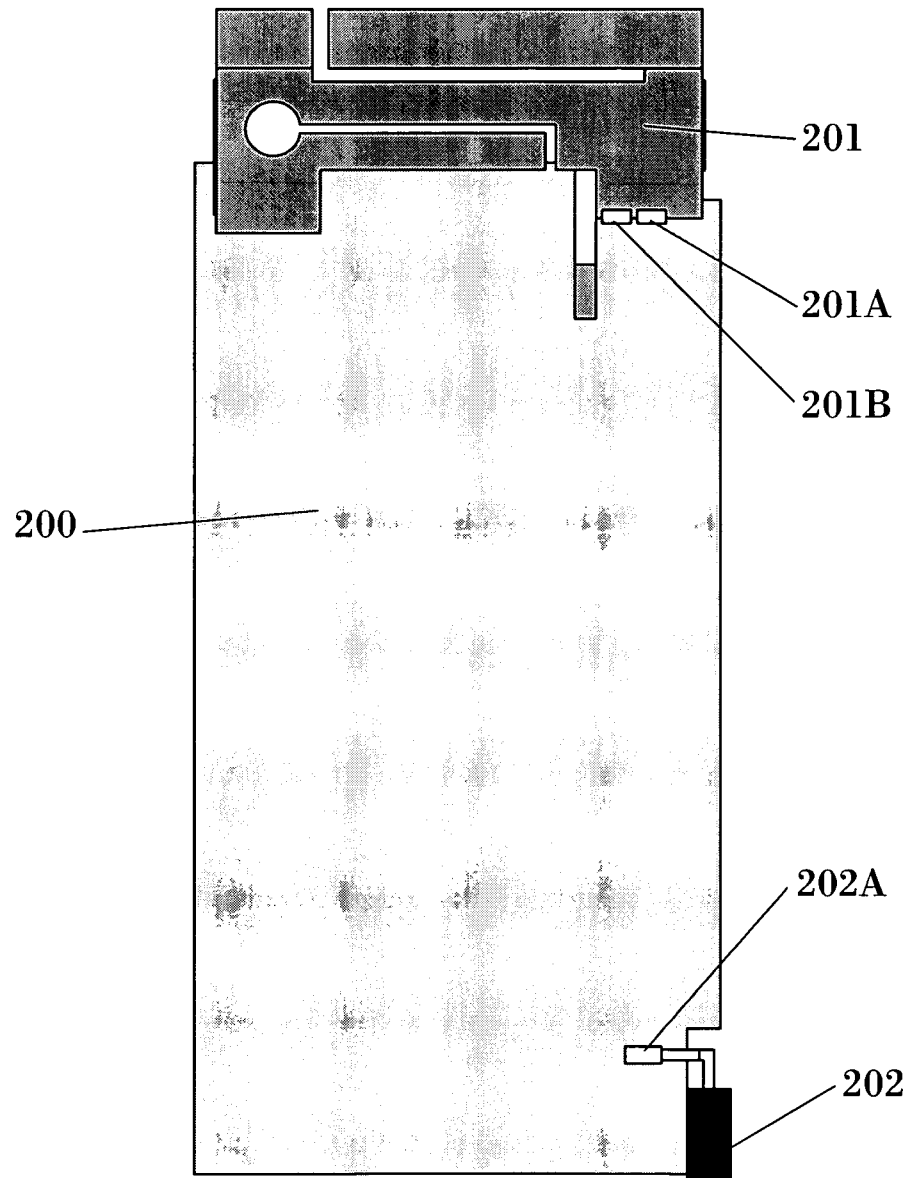
FIG. 2 (PRIOR ART)
