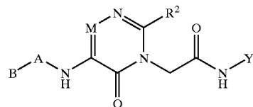
(I-EMPS wherein B is a non-aromatic cyclic substituent)
