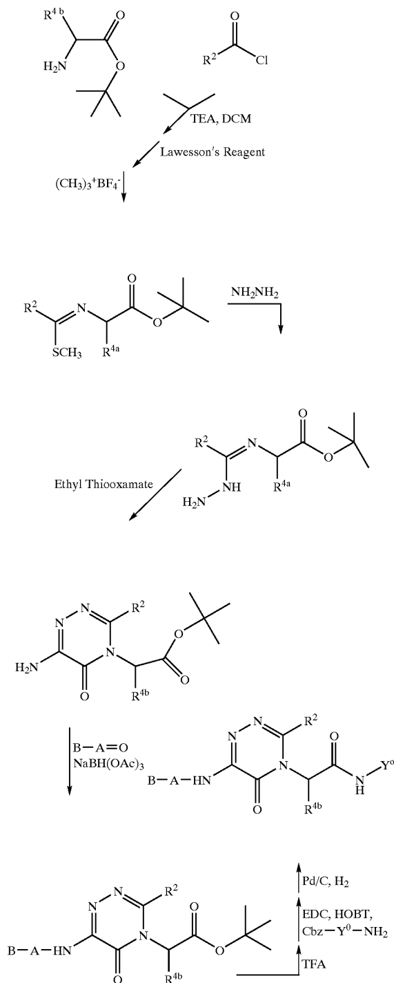
Scheme 9: General 4-AzaPyrimidinone Synthesis
