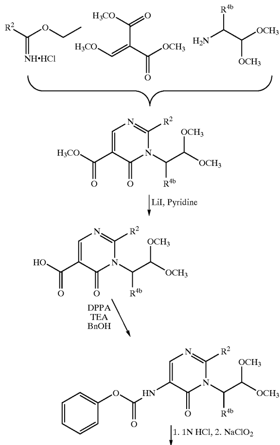
Scheme 1: General Pyrimidinon Synthesis-I
