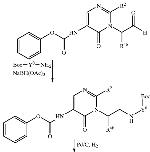
Scheme 8: General Methylene Pyrimidinone Synthesis
