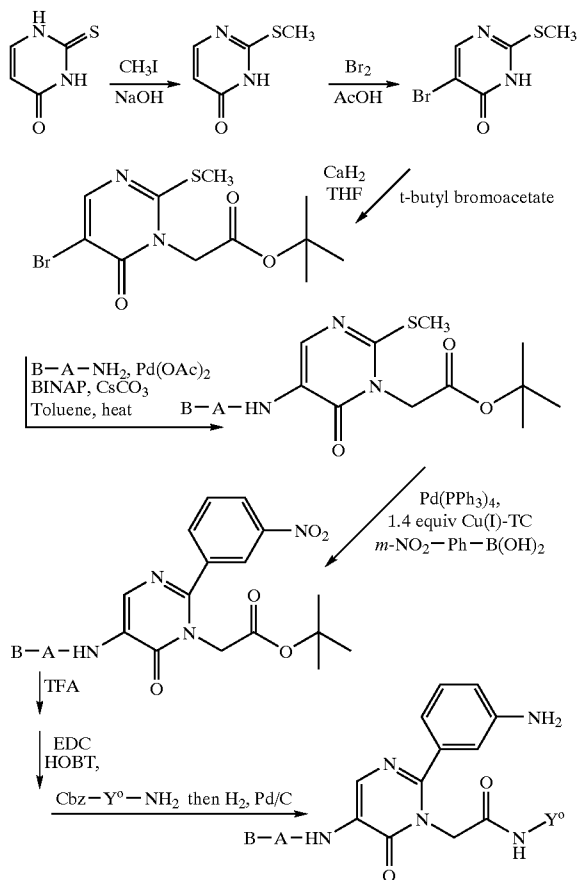
Scheme 7: Alternate Pyrimidinon Synthesis
