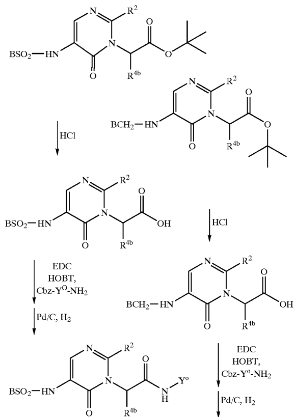
Scheme 5: General Pyrimidinone Synthesis-I (Concluded)
