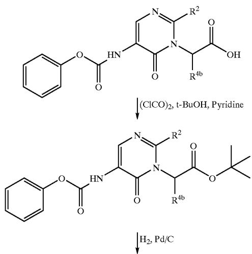
Scheme 2: General Pyrimidinone Synthesis-I (Continued)
