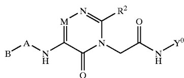
(I-MPS wherein B is a non-aromatic cyclic substituent)
