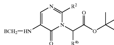
Scheme 4: General Pyrimidinone Synthesis-I (Concluded)
