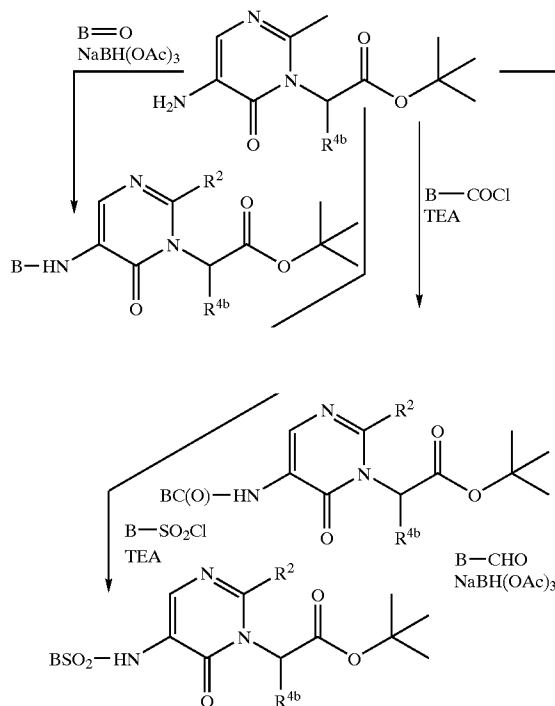
Scheme 3: General Pyrimidinone Synthesis-I (Continued)
