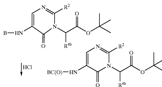
Scheme 4: General Pyrimidinone Synthesis-I (Concluded)
