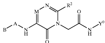
(I-EMPS wherein B is a non-cyclic substituent)
