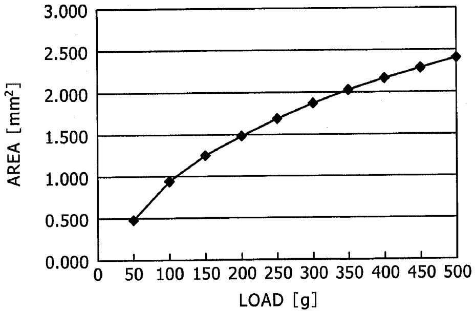
AREA-LOAD CHARACTERISTICS
