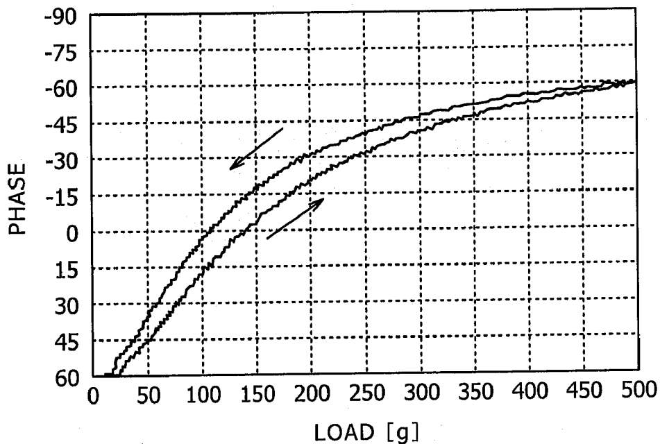
PHASE-LOAD CHARACTERISTICS
