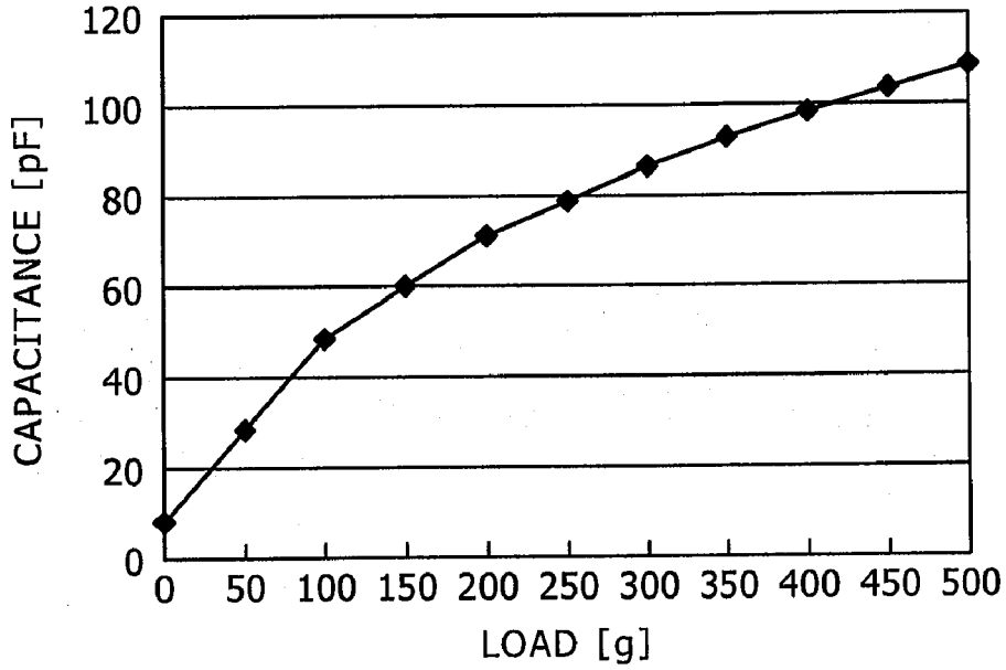
CAPACITANCE-LOAD CHARACTERISTICS
