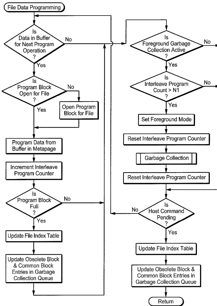
Flow Chart for Programming File Data
