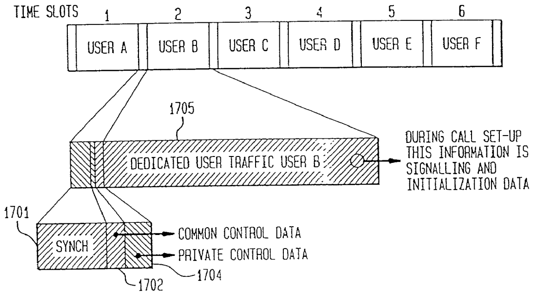
FIG. 17 SYNCH AND CONTROL CHANNEL STRUCTURE
