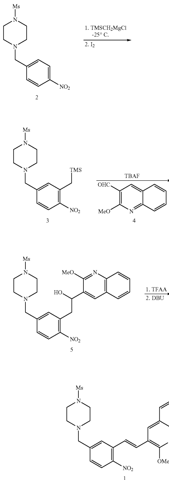
SCHEME 1
