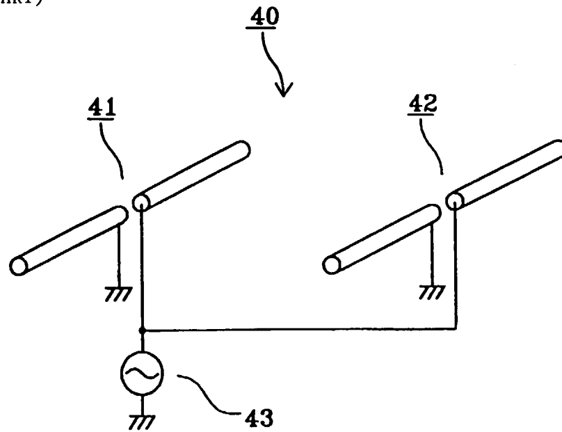
Fig. 6 (PRIOR ART)
