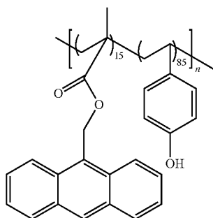
Synthesis Examples 2-5
