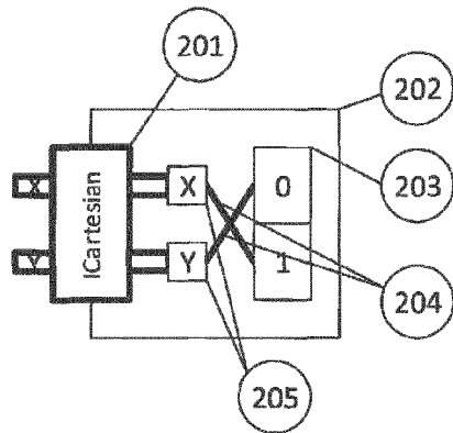
Figure 2: Dimension interface access space vector
