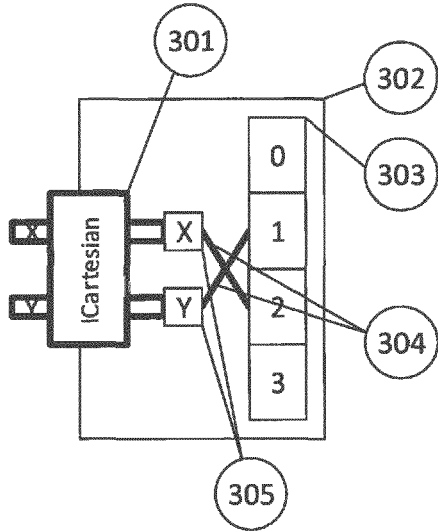
Figure 3: Dimension interface accesses different indexes of space vector
