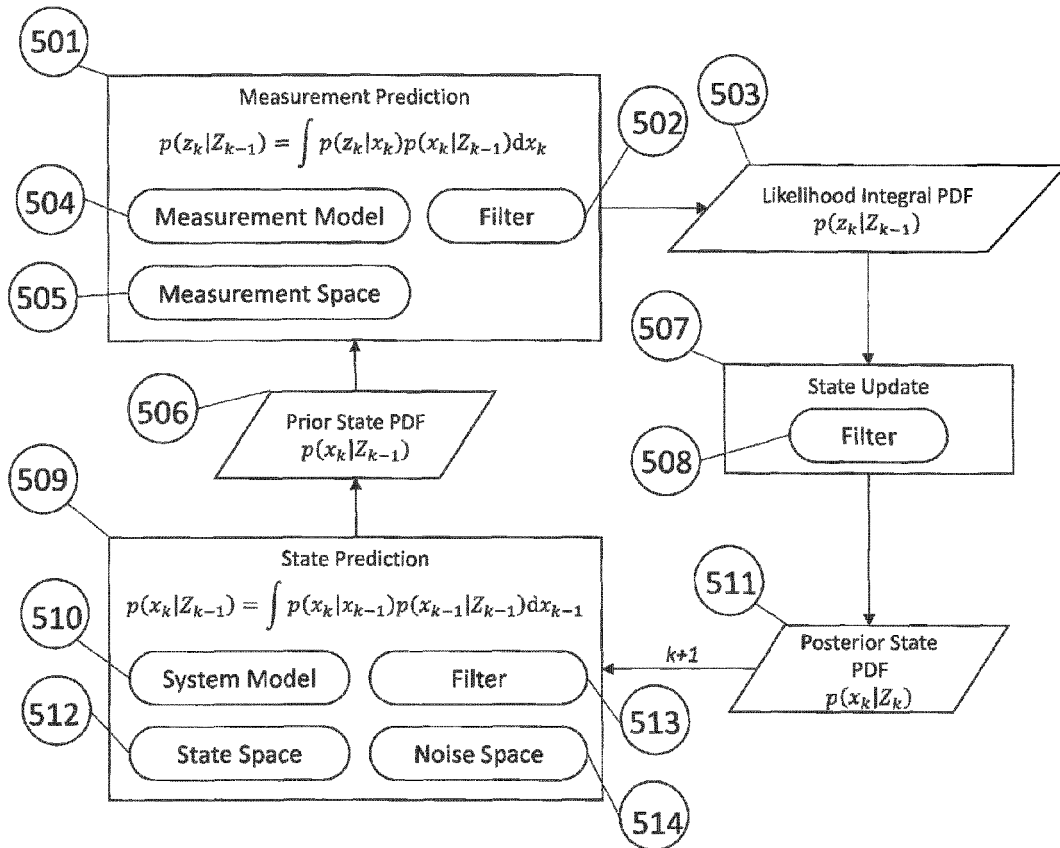
Figure 5: Bayes filter process including configurable spaces (505,512,514), models (504,510), and filters (502,508,513)
