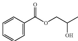
Propylene Glycol Mono-Benzoate
