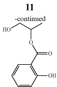
Propylene Glycol Mono-Salicylate
