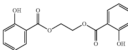
Ethylene Glycol Di-Salicylate
