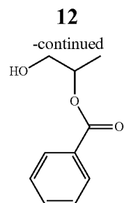
Propylene Glycol Mono-Benzoate
