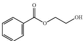
Ethylene Glycol Mono-Benzoate
