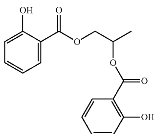
Propylene Glycol Di-Salicylate
