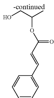
Propylene Glycol Mono-Cinnamate
