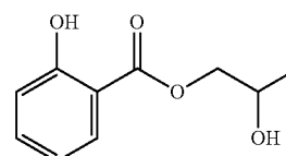
Propylene Glycol Mono-Salicylate
