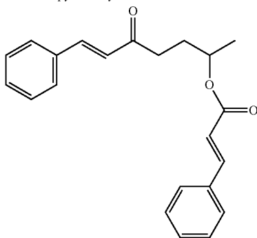
Propylene Glycol Di-Cinnamate
