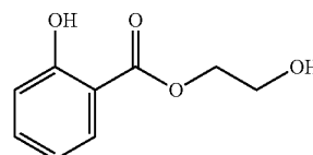
Ethylene Glycol Mono-Salicylate
