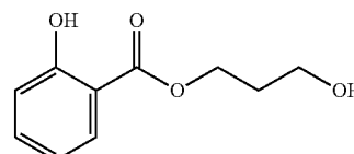
Propylene Glycol Mono-Salicylate
