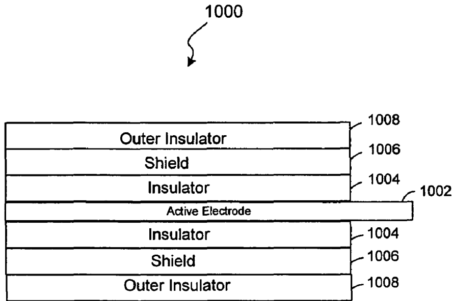
Electrode Assembly
