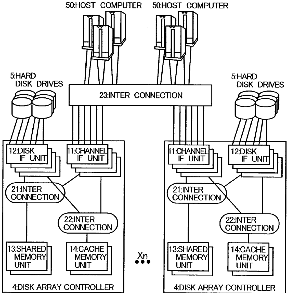
FIG.4 (PRIOR ART)
