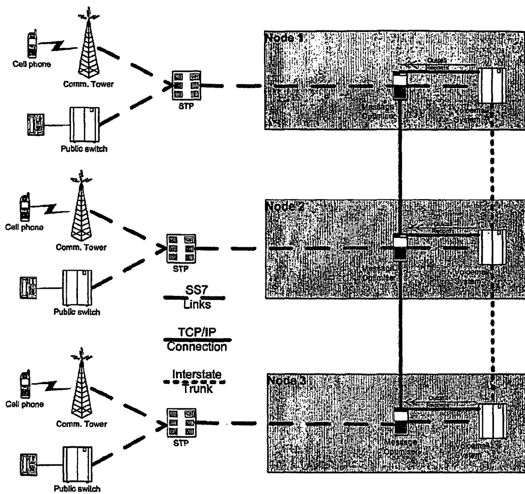
Message Optimiser™ Network Topology - Option A
