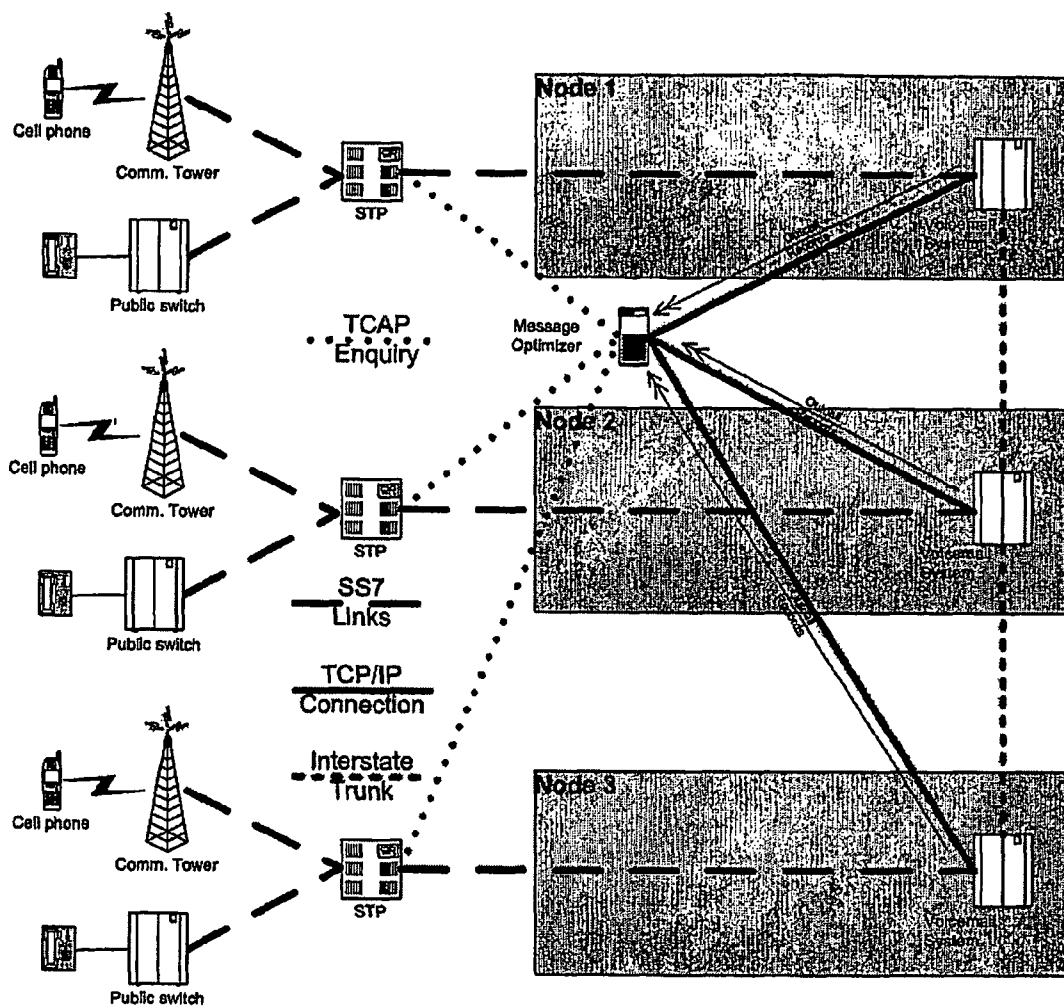
Message Optimise Network Topology – Option B
