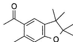
2,2,3,3,6-Pentamethyl-5-acetylcoumaran
