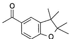
2,2,3,3-Tetramethyl-5-acetylcoumaran
