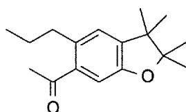
2,2,3,3-Tetramethyl-5-propyl-6-acetylcoumaran
