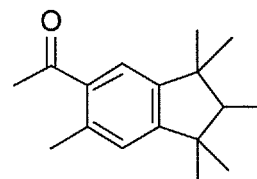
Phantolide (PFW)
