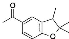
2,2,3-Trimethyl-5-acetylcoumaran
