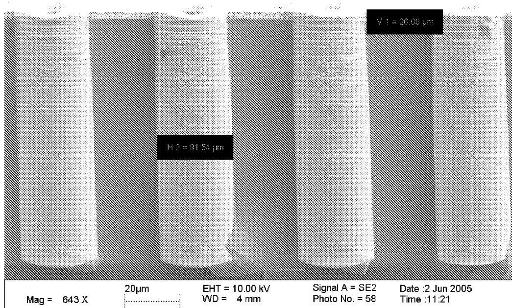
20 µm diameter 100µm deep filled Via
