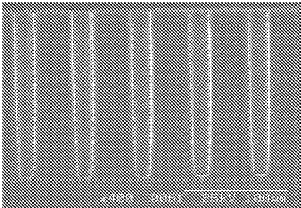
20µm diameter ~ 150µm deep
