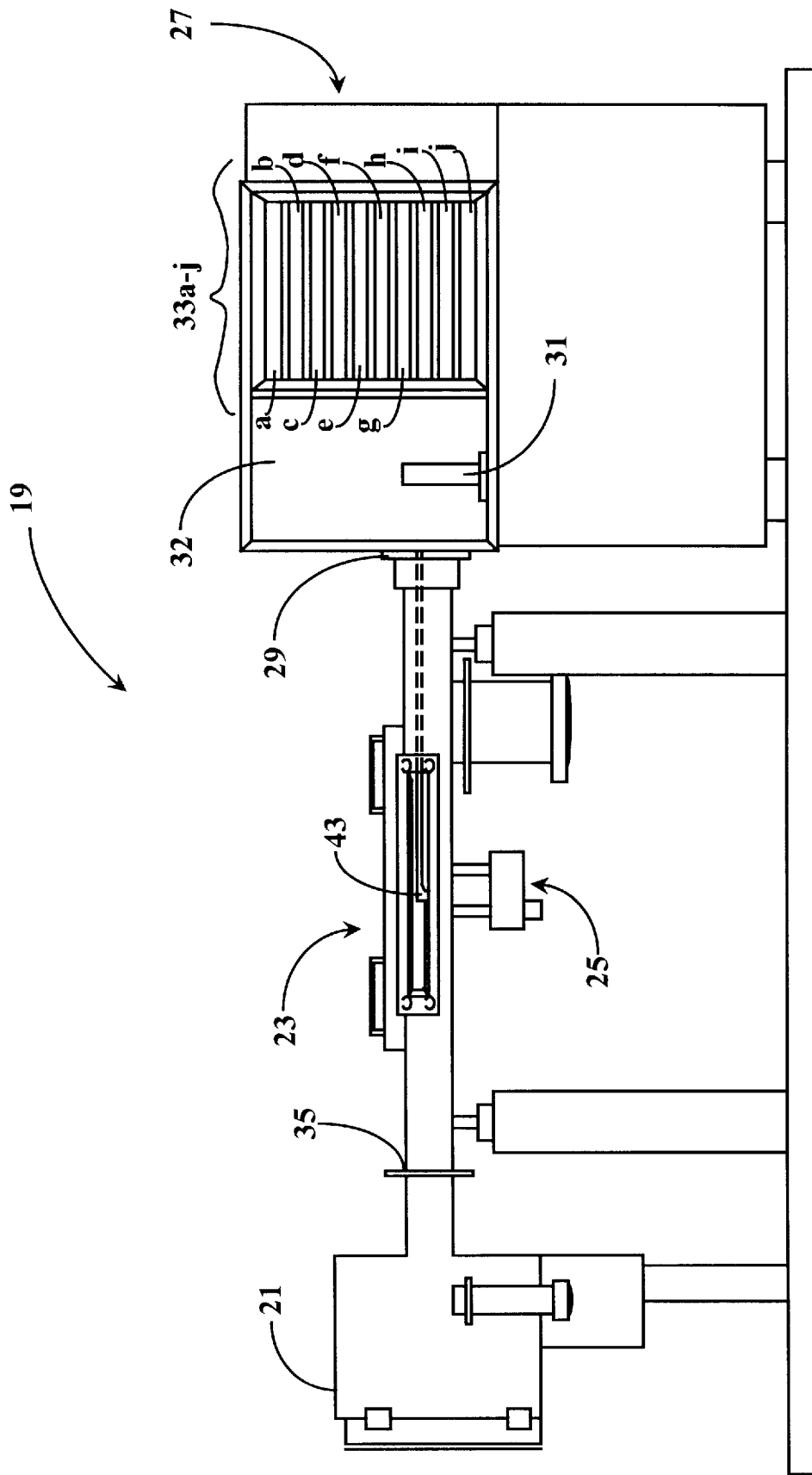
Vertically Stacked Compact ALD Reactor (VESCAR) System
