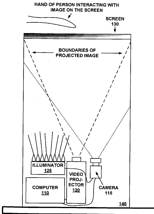
BASIC HARDWARE CONFIGURATION
