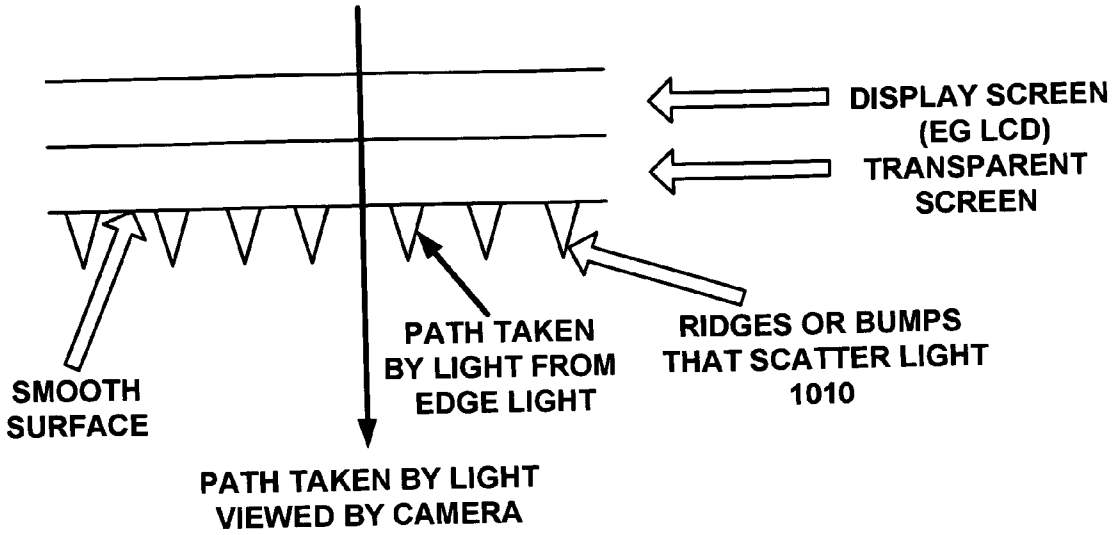
CROSS SECTION OF SCREEN WITH MICROSCOPIC SCATTERING RIDGES OR BUMPS (NOT TO SCALE)
