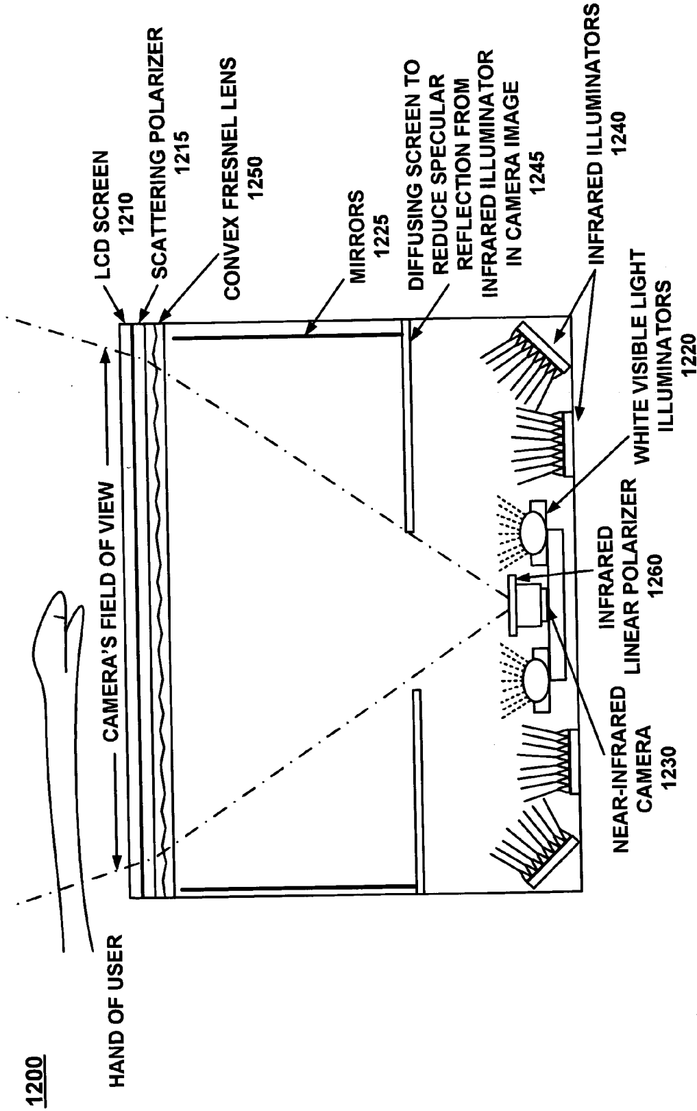
FLAT PANEL DISPLAY CROSS-SECTION
