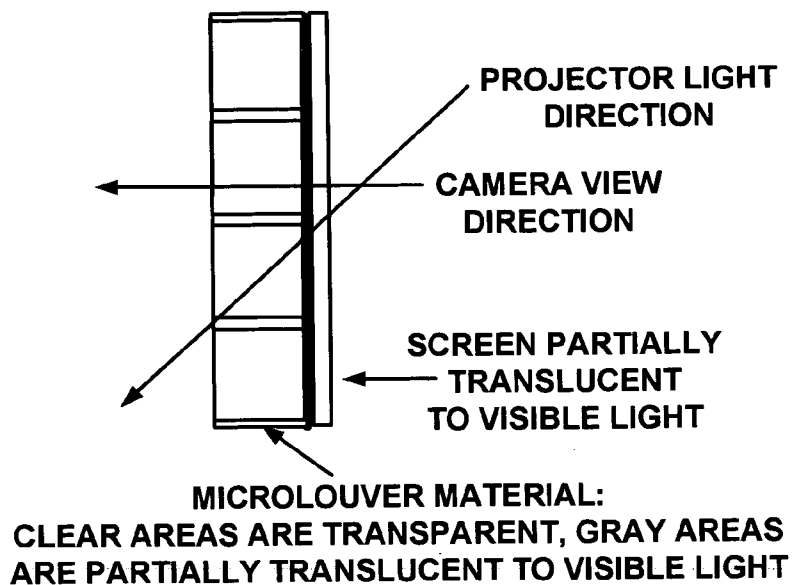
CLOSE-UP OF MICROLOUVER SCREEN SECTION
