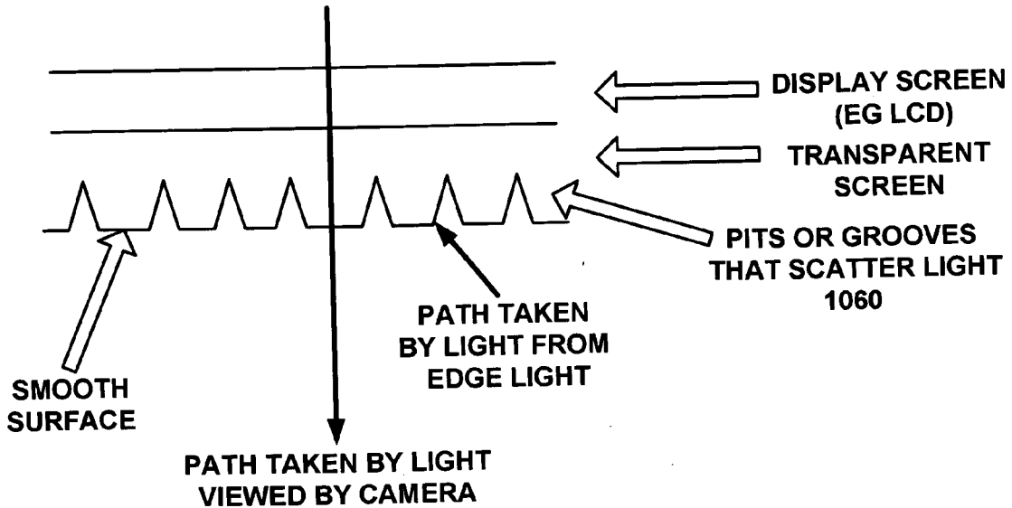
CROSS SECTION OF SCREEN WITH MICROSCOPIC SCATTERING PITS OR GROOVES (NOT TO SCALE)
