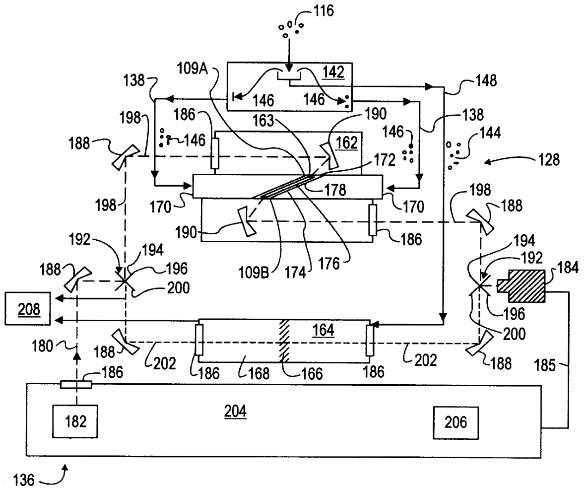
FIG. 6 PRIOR ART
