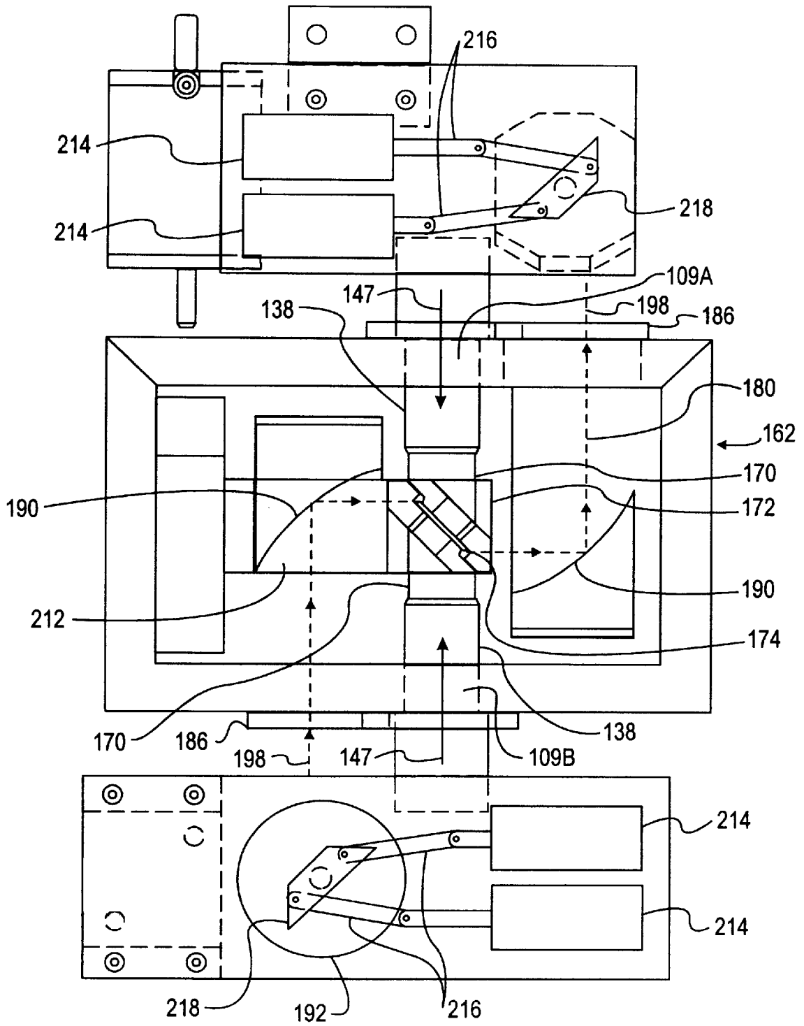
FIG. 7 PRIOR ART
