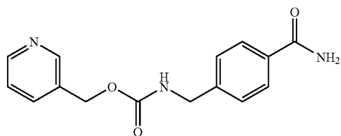
Pyridin-3-ylmethyl{[4-(aminocarbonyl)phenyl]methyl}carbamate
