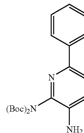
Di-tert-butyl(3-amino-6-phenylpyridin-2-yl)imidodicarbonate
