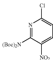
Di-tert-butyl(6-chloro-3-nitropyridin-2-yl)imidodicarbonate
