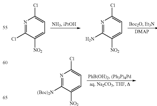
Scheme 10
