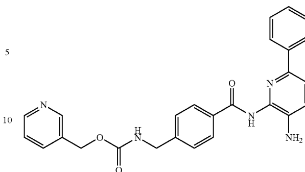
Pyridin-3-ylmethyl{[4-({[3-amino-6-phenylpyridin-2-yl]amino]carbonyl]phenyl]methyl]carbamate
