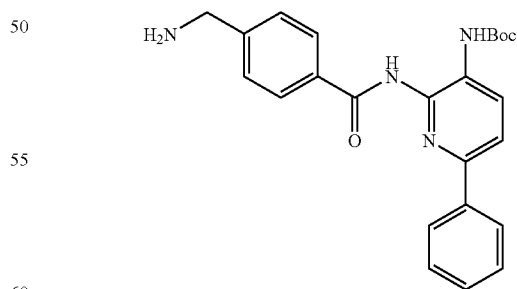
Tert-butyl(2-([4-(aminomethyl)benzoyl]amino)-6-phenylpyridin-3-yl)carbamate
