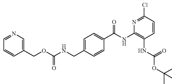
Pyridin-3-ylmethyl{[4-({[6-chloro-3-({[1,1-dimethylethyl]oxy)carbonyl]amino}pyridin-2-yl]amino}carbonyl)phenyl]methyl}carbamate
