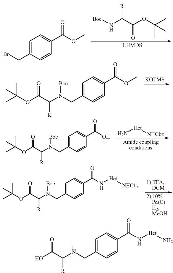
Scheme 8
