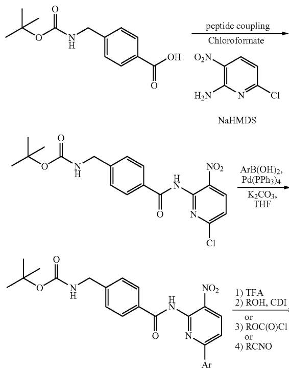
Scheme 15
