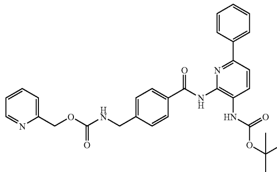
Pyridin-2-ylmethyl{4-[(3-[(tert-butoxycarbonyl)amino]-6-phenylpyridin-2-yl)amino]carbonyl}benzyl}carbamate
