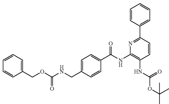
Benzyl{4-[(3-[(tert-butoxycarbonyl)amino]-6-phenylpyridin-2-yl)amino]carbonyl}benzyl}carbamate
