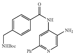
tert-Butyl(4-((3-amino-6-phenylpyridin-4-yl)amino)carbonyl)benzyl)carbamate
