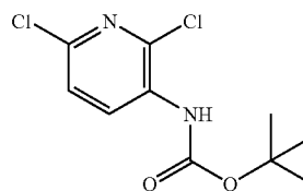
1,1-dimethylethyl(2,6-dichloropyridin-3-yl)carbamate
