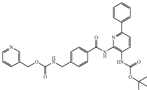
1,1-dimethylethyl{6-phenyl-2-[(4-[(pyridin-3-ylmethyl)oxy]carbonyl]amino)methyl]phenyl]carbonyl]amino]pyridin-3-yl]carbamate
