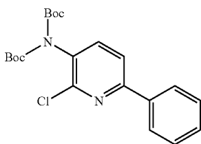
Di-tert-butyl(2-chloro-6-phenylpyridin-3-yl)imidodicarbonate
