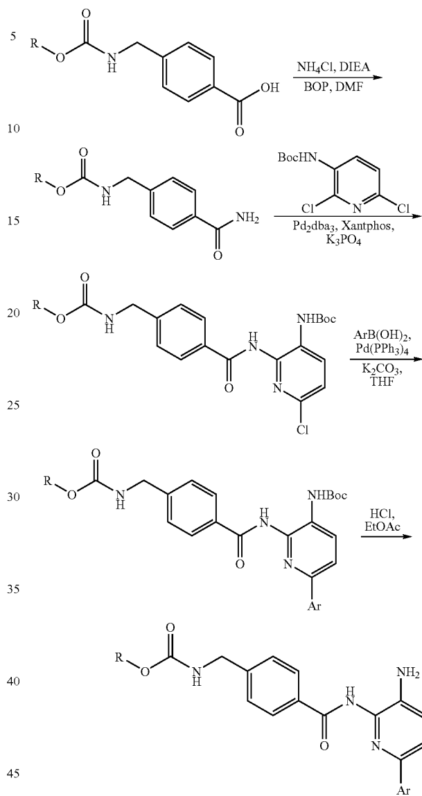
Scheme 9
