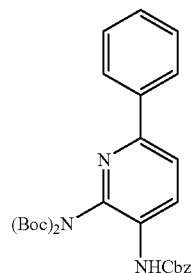
Di-tert-butyl(3-((benzyloxy)carbonylamino)-6-phenylpyridin-2-yl)imidodicarbonate
