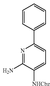
Benzyl(2-amino-6-phenylpyridin-3-yl)carbamate
