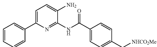
Methyl(4-[[[(3-amino-6-phenylpyridin-2-yl)amino]carbonyl]benzyl]carbamate
