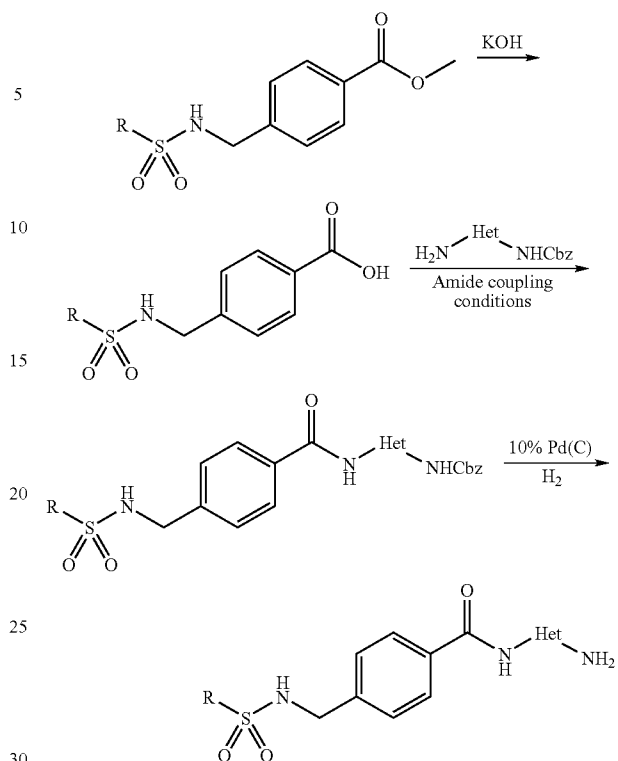
Scheme 6
