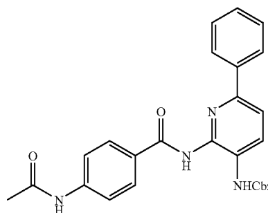
Benzyl(2-[[4-(acetylamino)benzoyl]amino]-6-phenylpyridin-3-yl)carbamate
