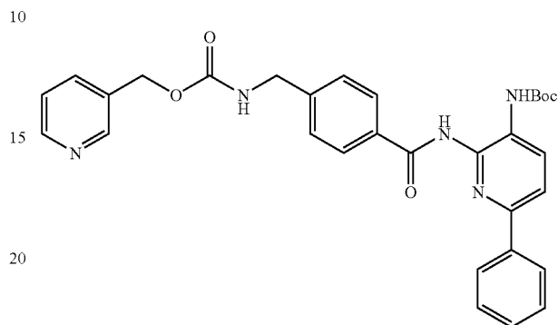
Pyridin-3-ylmethyl{4-((3-[(tert-butoxycarbonyl)amino]-6-phenylpyridin-2-yl)amino)carbonyl}benzyl)carbamate
