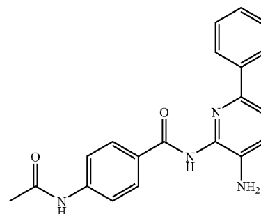
4-(Acetylamino)-N-(3-amino-6-phenylpyridin-2-yl)benzamide
