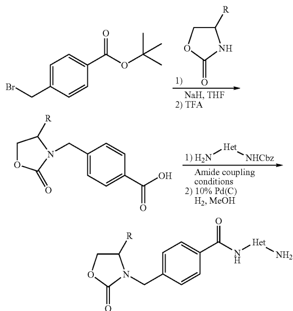
Scheme 7
