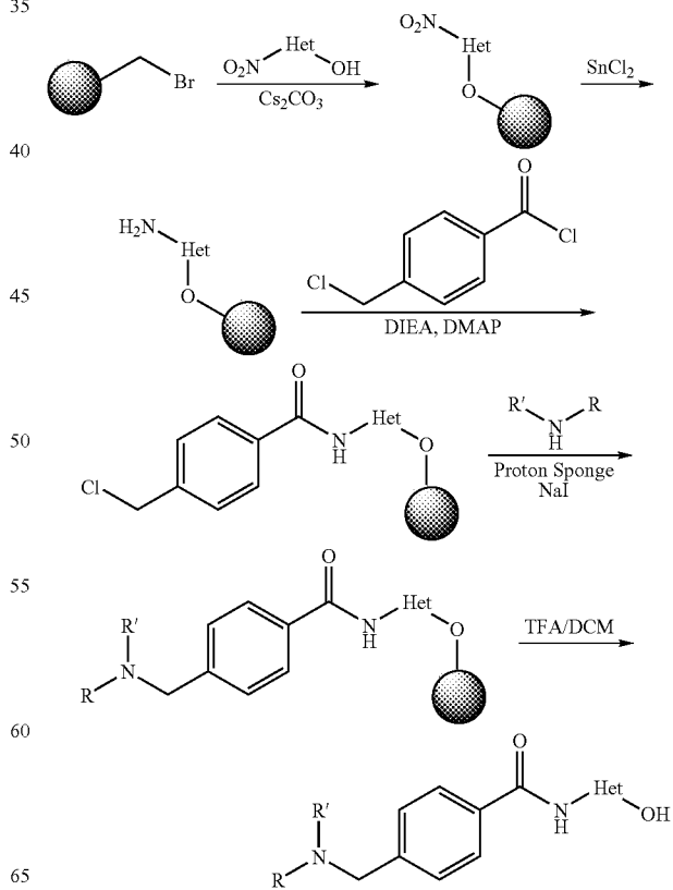
Scheme 6
