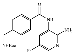
tert-Butyl(4-[[2-amino-5-phenylpyridin-3-yl]amino]carbonyl)benzyl)carbamate
