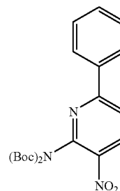
Di-tert-butyl(3-nitro-6-phenylpyridin-2-yl)imidodicarbonate
