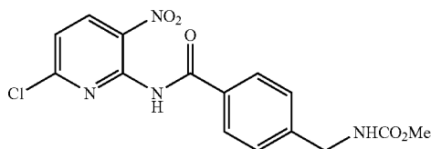
Methyl(4-[[[(6-chloro-3-nitropyridin-2-yl)amino]carbonyl]benzyl]carbamate
