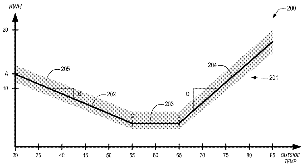
COARSE-GRAINED 5-PARAMETER REGRESSION BASELINE MODEL
