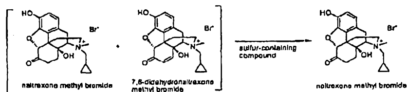
Reaction Scheme 9
