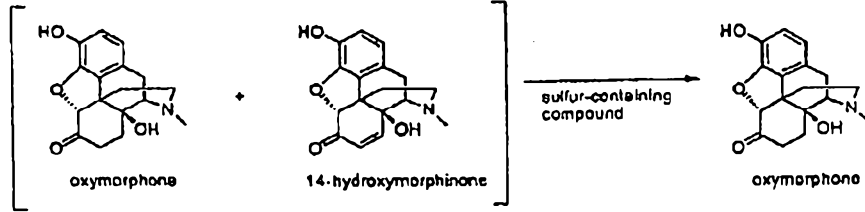
Reaction Scheme 4
