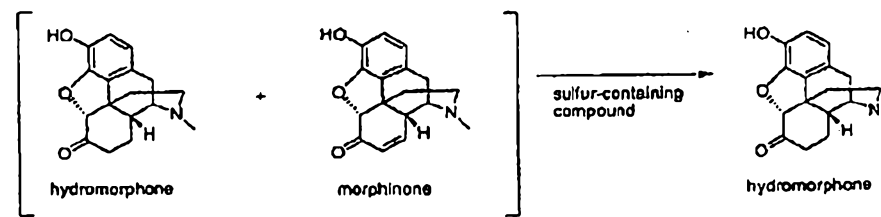
Reaction Scheme 6
