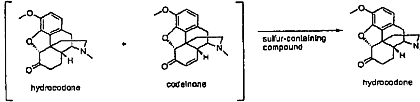
Reaction Scheme 3
