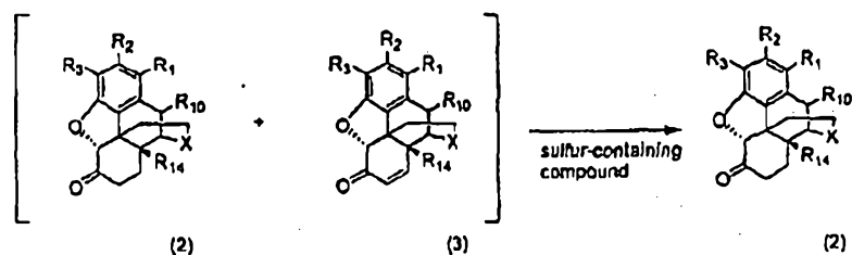
Reaction Scheme 11
