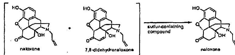
Reaction Scheme 9
