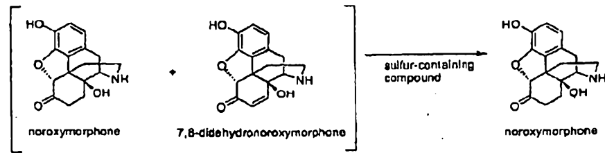
Reaction Scheme 5
