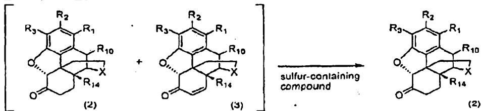
Reaction Scheme 2
