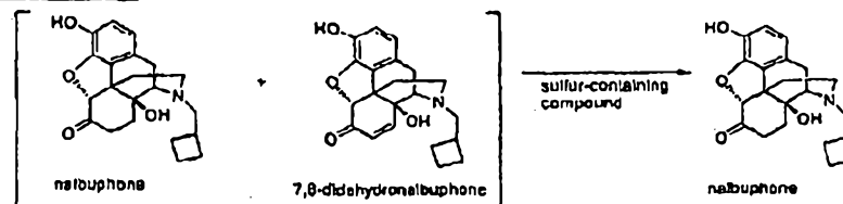
Reaction Scheme 10
