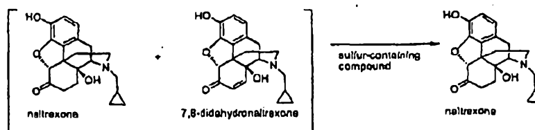
Reaction Scheme 8
