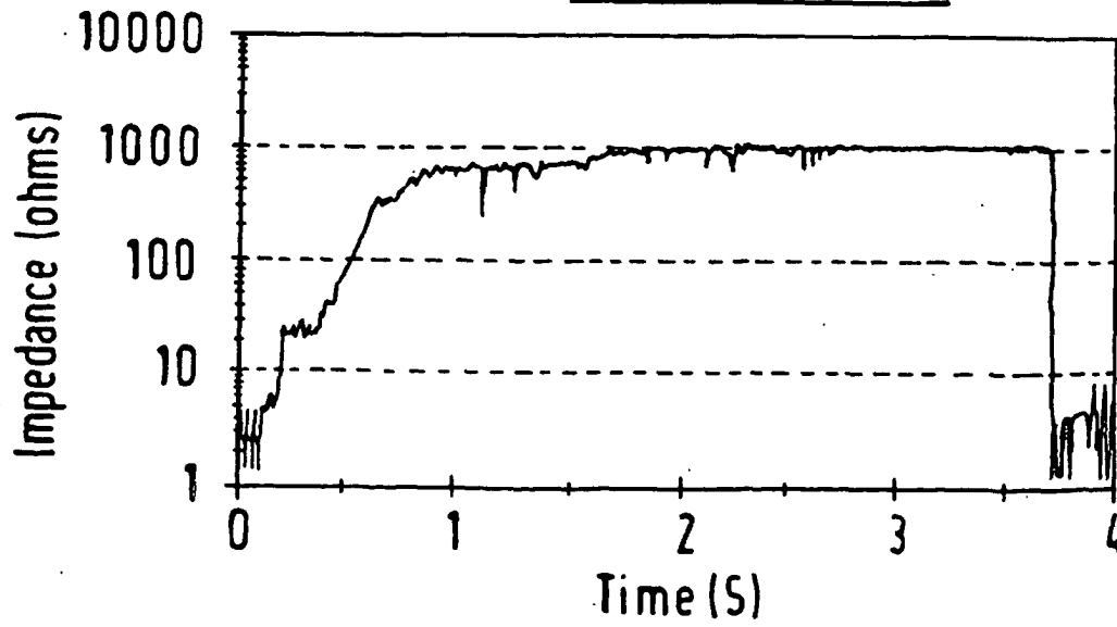
FIG. 2(b) IMPEDANCE
