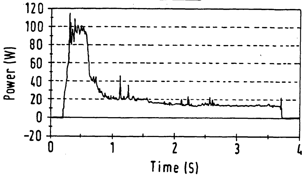
FIG. 2(a) POWER
