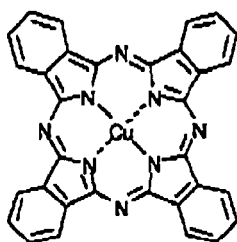
Compound A
