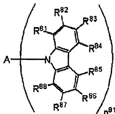
Formula (VIII)
