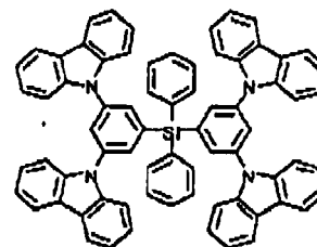
Comparative Compound 9
