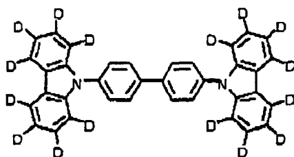
Exemplified Compound (1-3)
