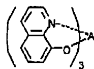
Compound D
