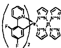
Light-Emitting Material E (460 nm)
