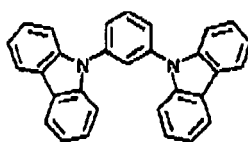
Comparative Compound 2
