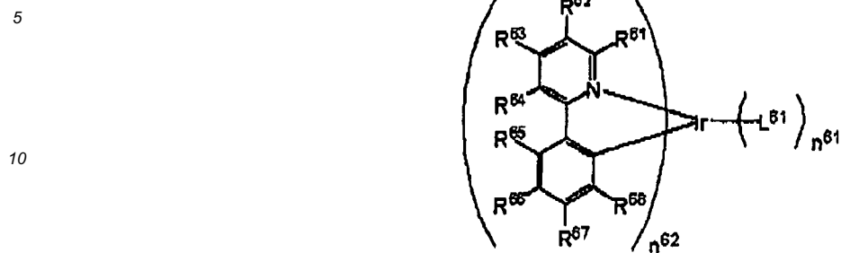
Formula (VI)
