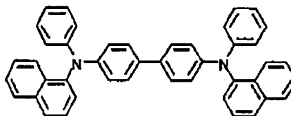
Compound B
