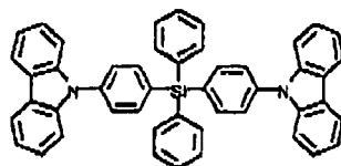
Comparative Compound 8
