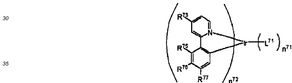
Formula (VII)
