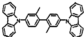
Comparative Compound 4
