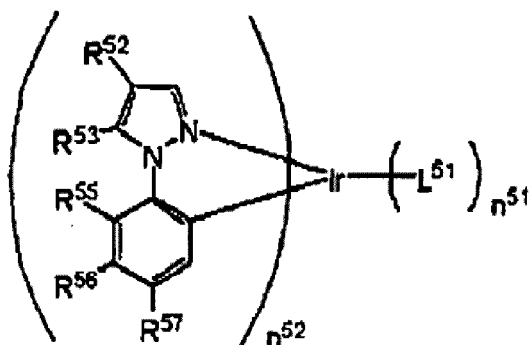
Formula (V)
