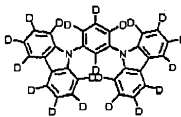
Exemplified Compound (4-6)
