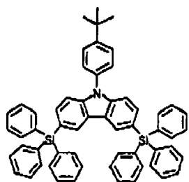
Comparative Compound 7
