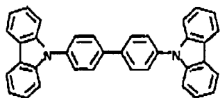
Comparative Compound 1
