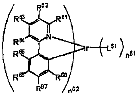
Formula (VI)
