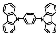
Comparative Compound 5
