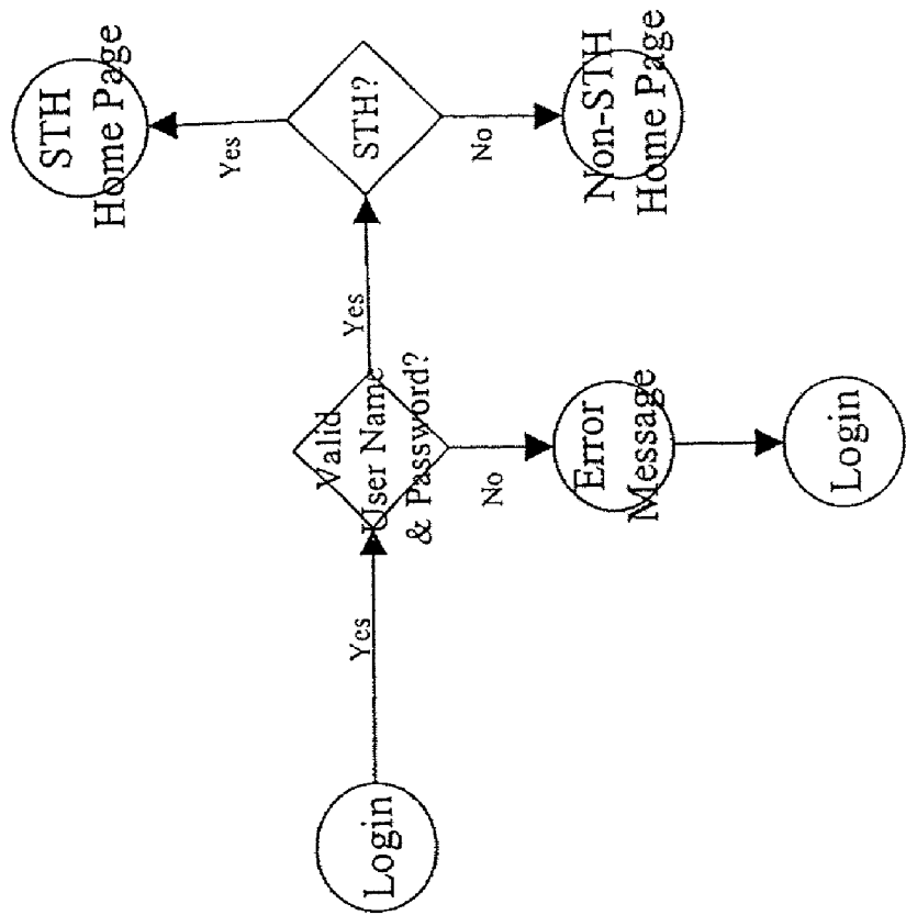
Figure 3 Login
