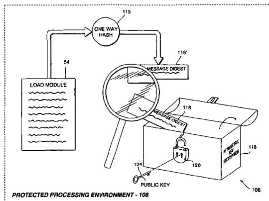
Authenticating a Digital Signature
