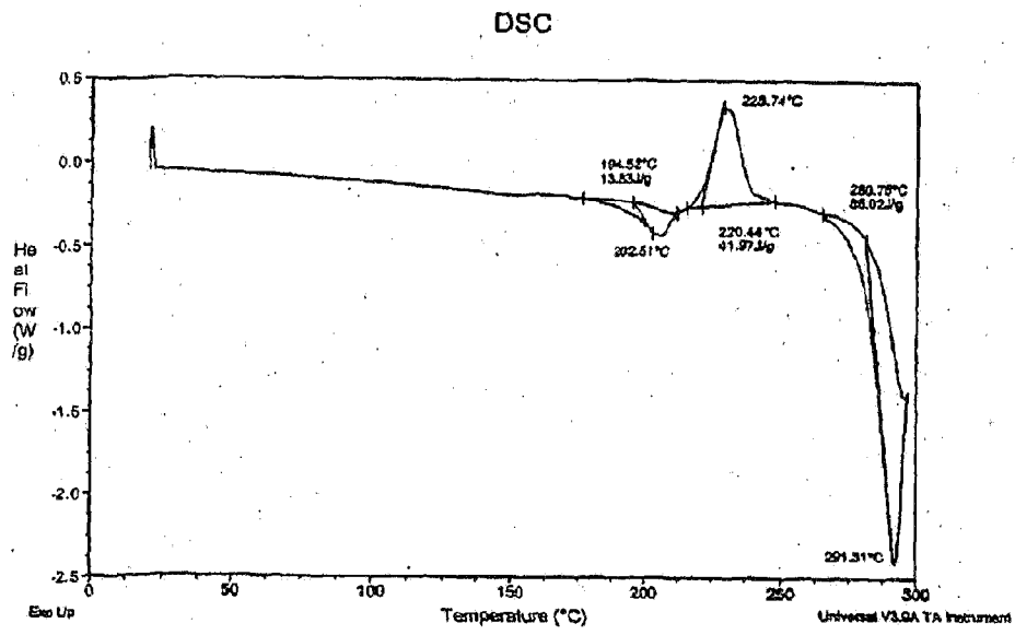
FIG. 3 DSC Trace of Compound 1
