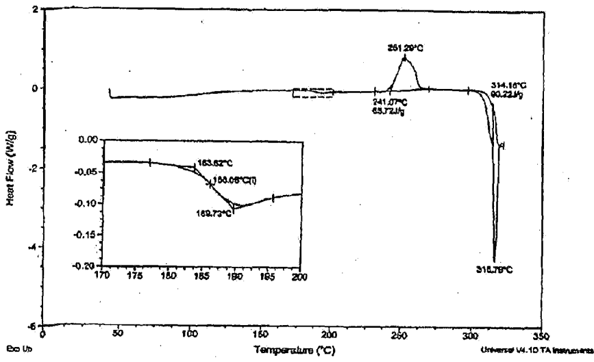
FIG. 13 DSC Trace of Amorphous Form
