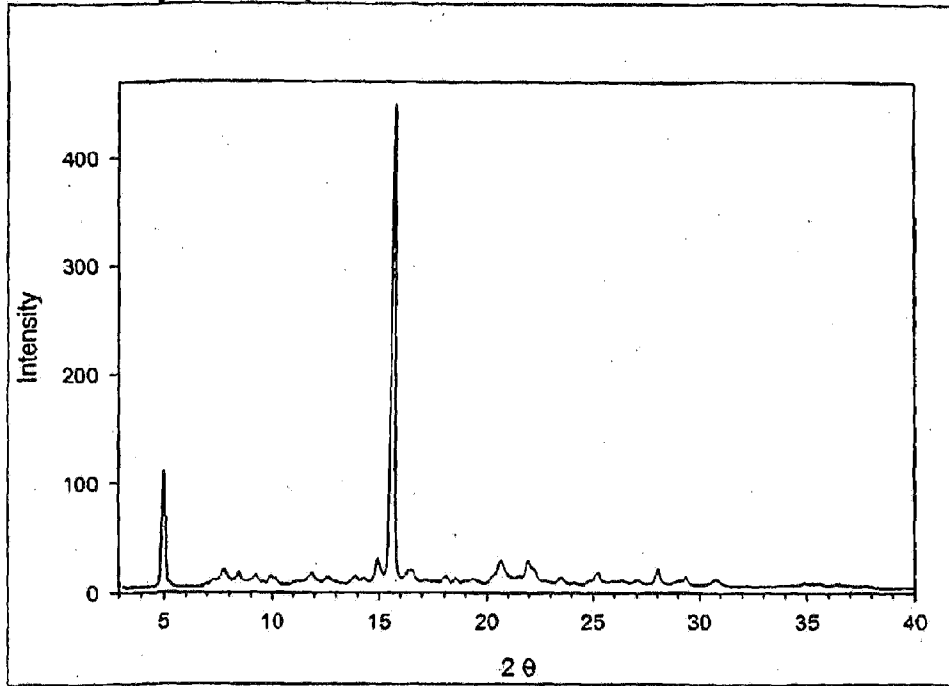
Figure 4 Powder X-Ray Diffraction pattern of Form A:
