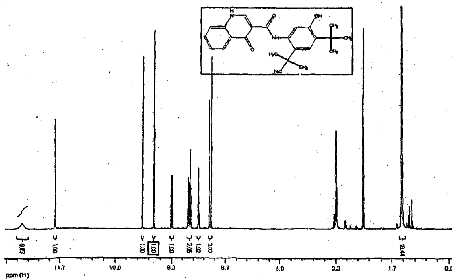
FIG. 2 1 H NMR Spectrum of Compound 1
