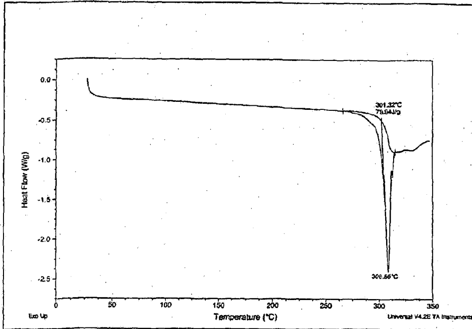
Figure 5 DSC trace of Form A:
