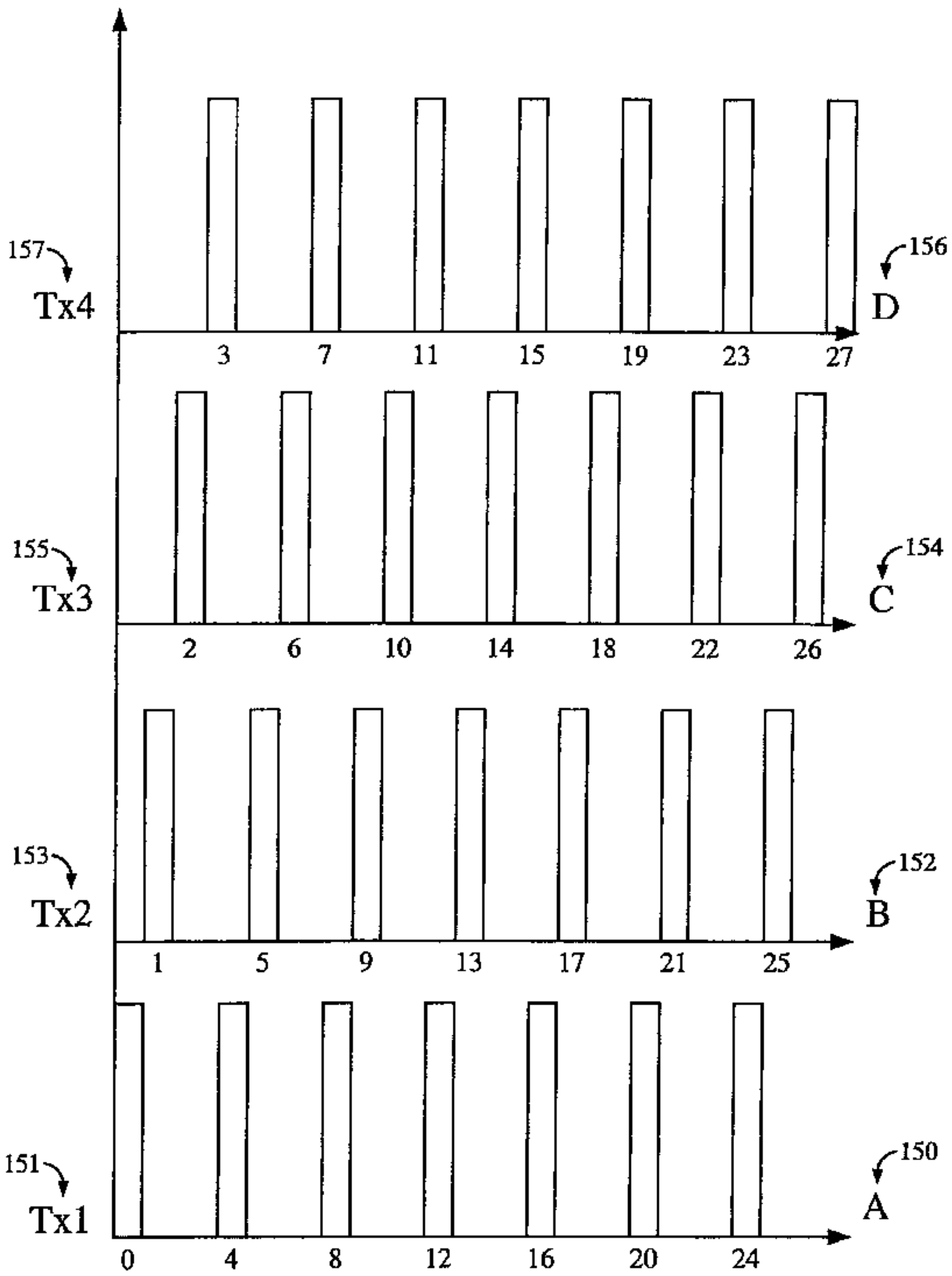
OFDM SUB-CHANNELS
