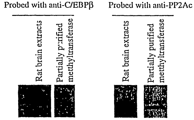
Figure 14 - C/EBP \beta and PP2Ac are components of isolated Methyltransferase activity
