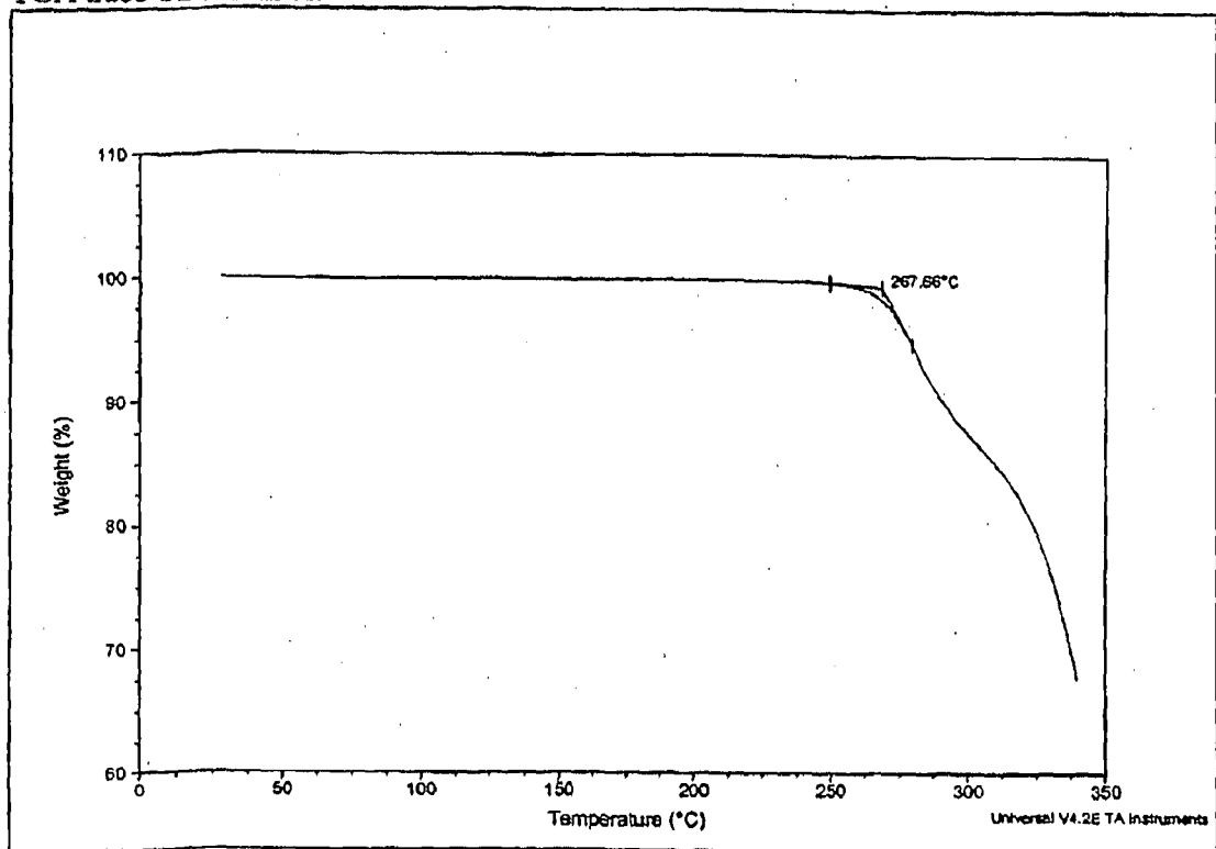
TGA trace of Form A:
