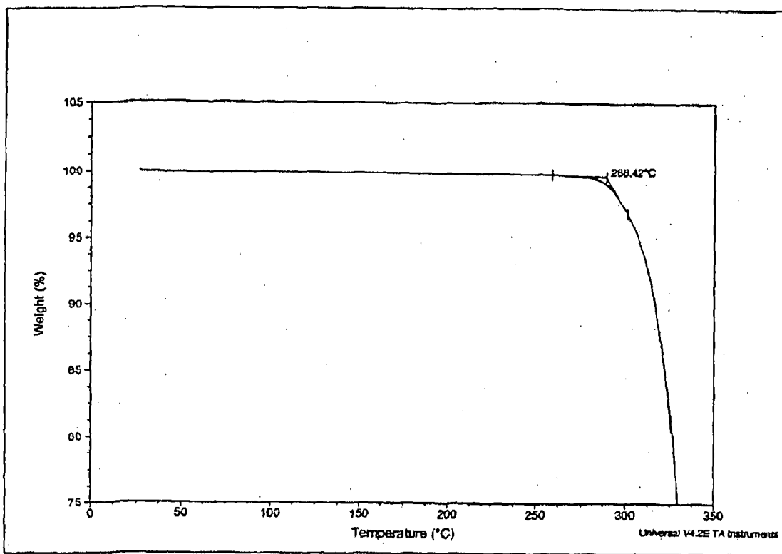
TGA trace of Form B:
