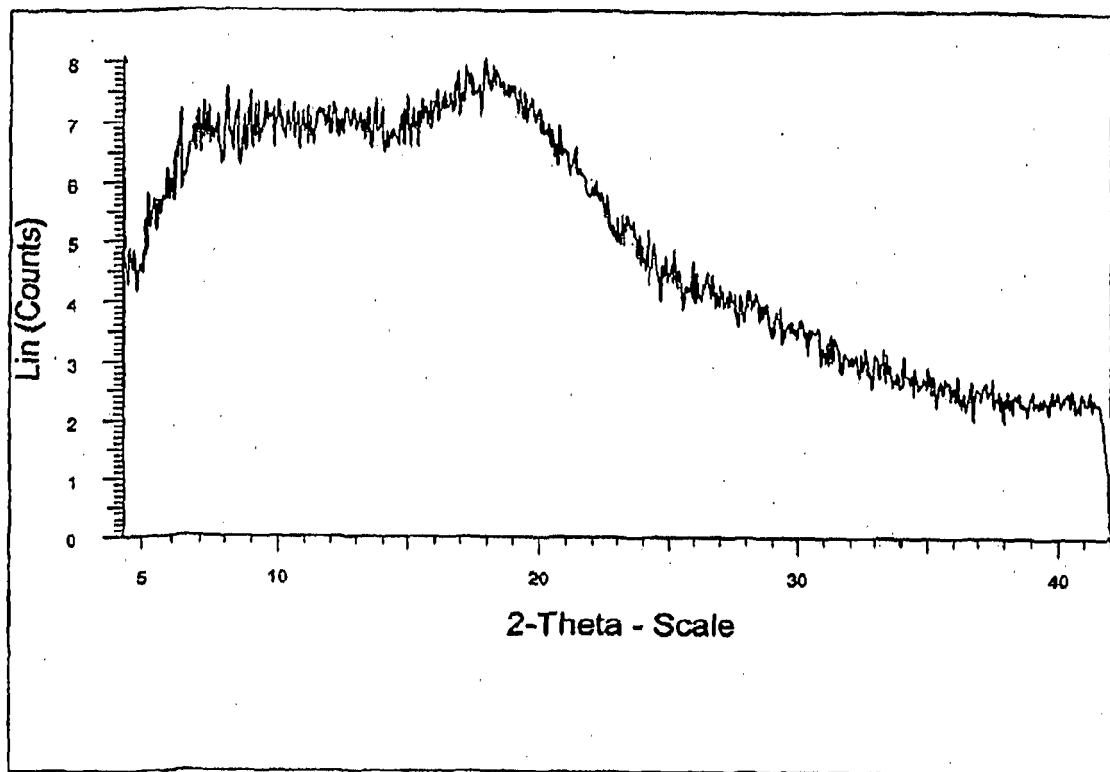
Figure 11: PXRD pattern of Amorphous Compound 1
