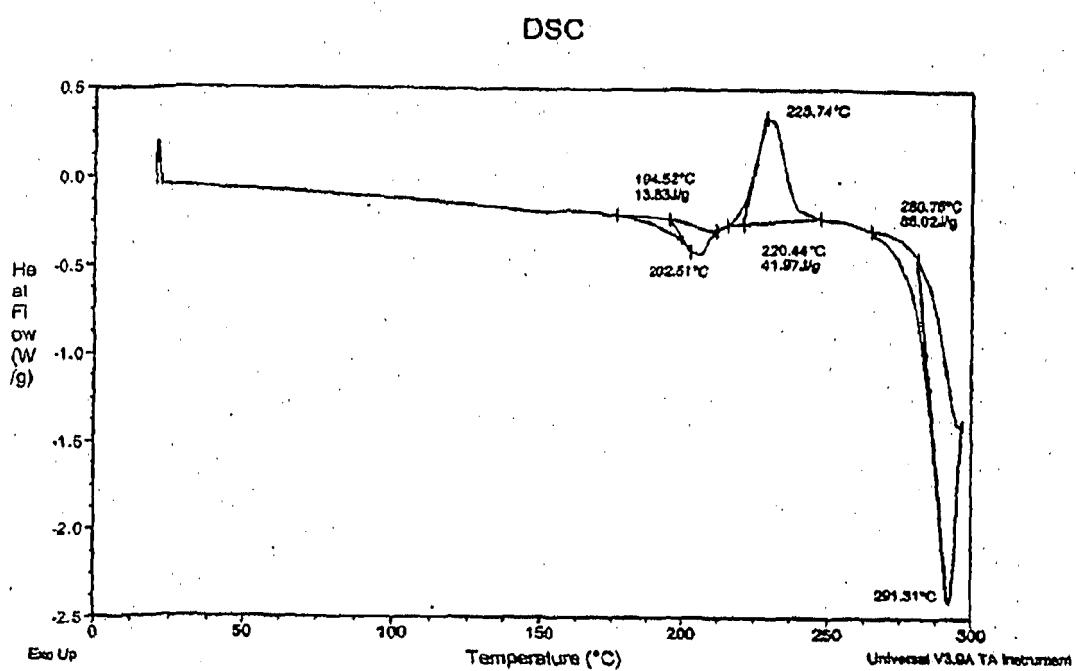
FIG. 3 DSC Trace of Compound 1
