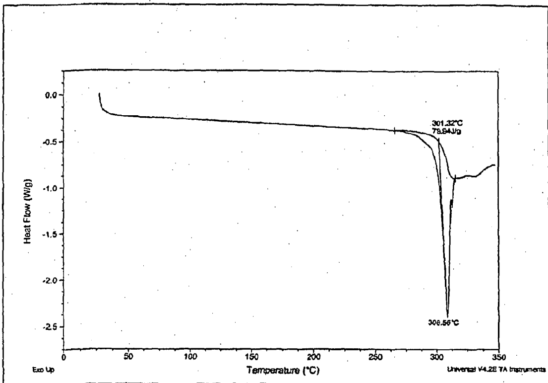
Figure 5 DSC trace of Form A:
