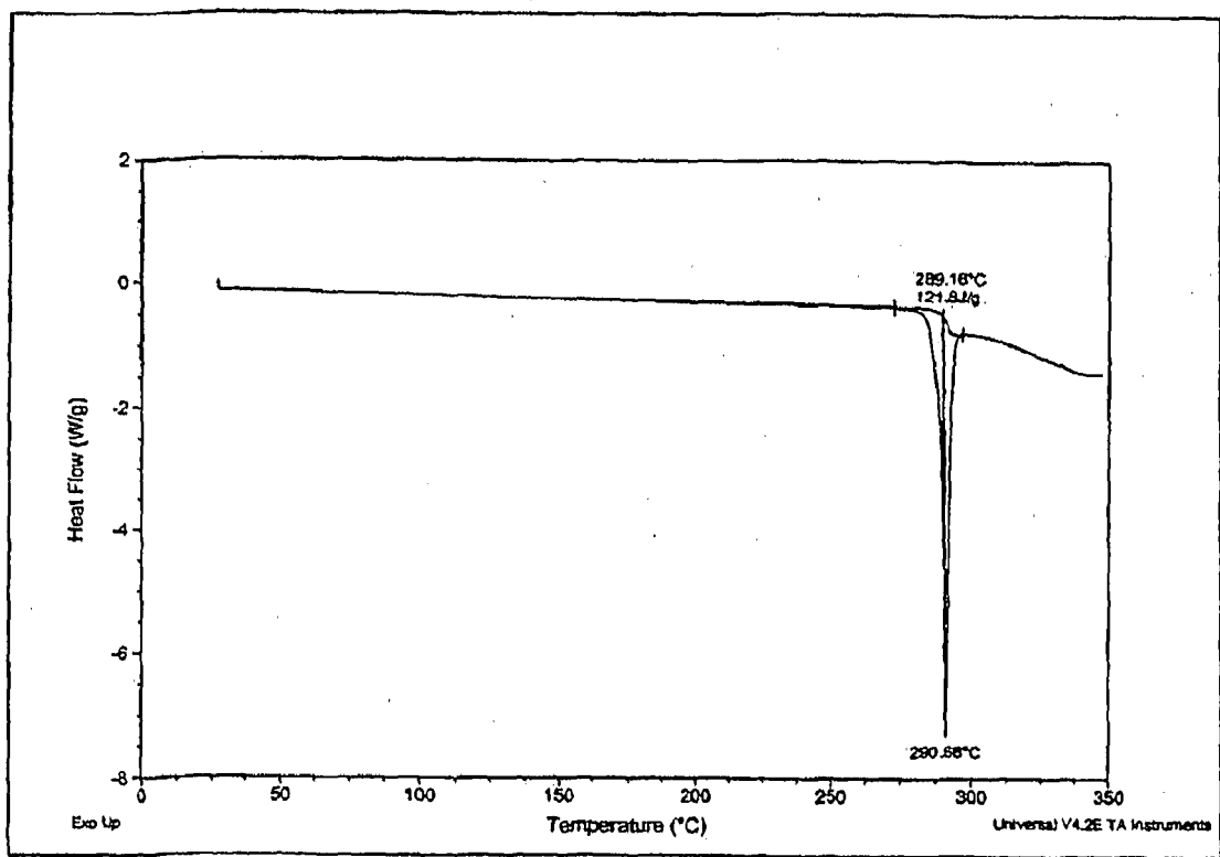
DSC trace of Form B:
