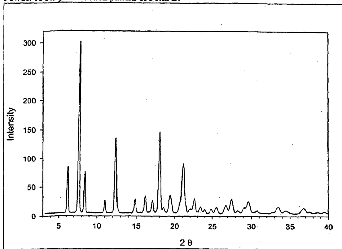
Powder X-Ray Diffraction pattern of Form B:
