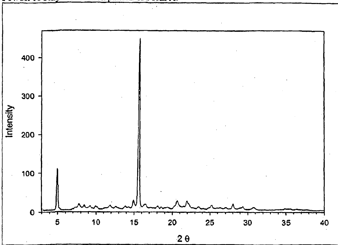
Figure 4 Powder X-Ray Diffraction pattern of Form A:
