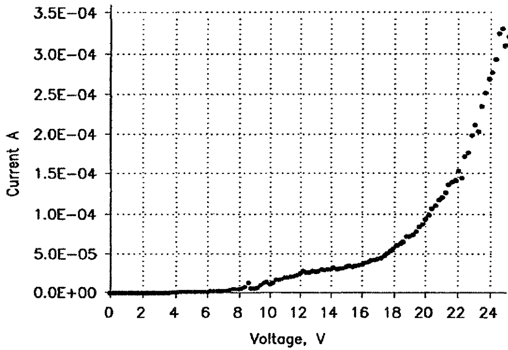
I-V characteristic of the device.
