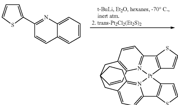
Scheme 10: Synthesis of cis-bis[2-(2'-thienyl)quinolinato-N,C 3 ] platinum (II).
