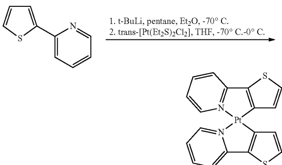
Scheme 9: Synthesis of cis-bis[2-(2'-thienyl)pyridinato-N,C 3 ] platinum (II).
