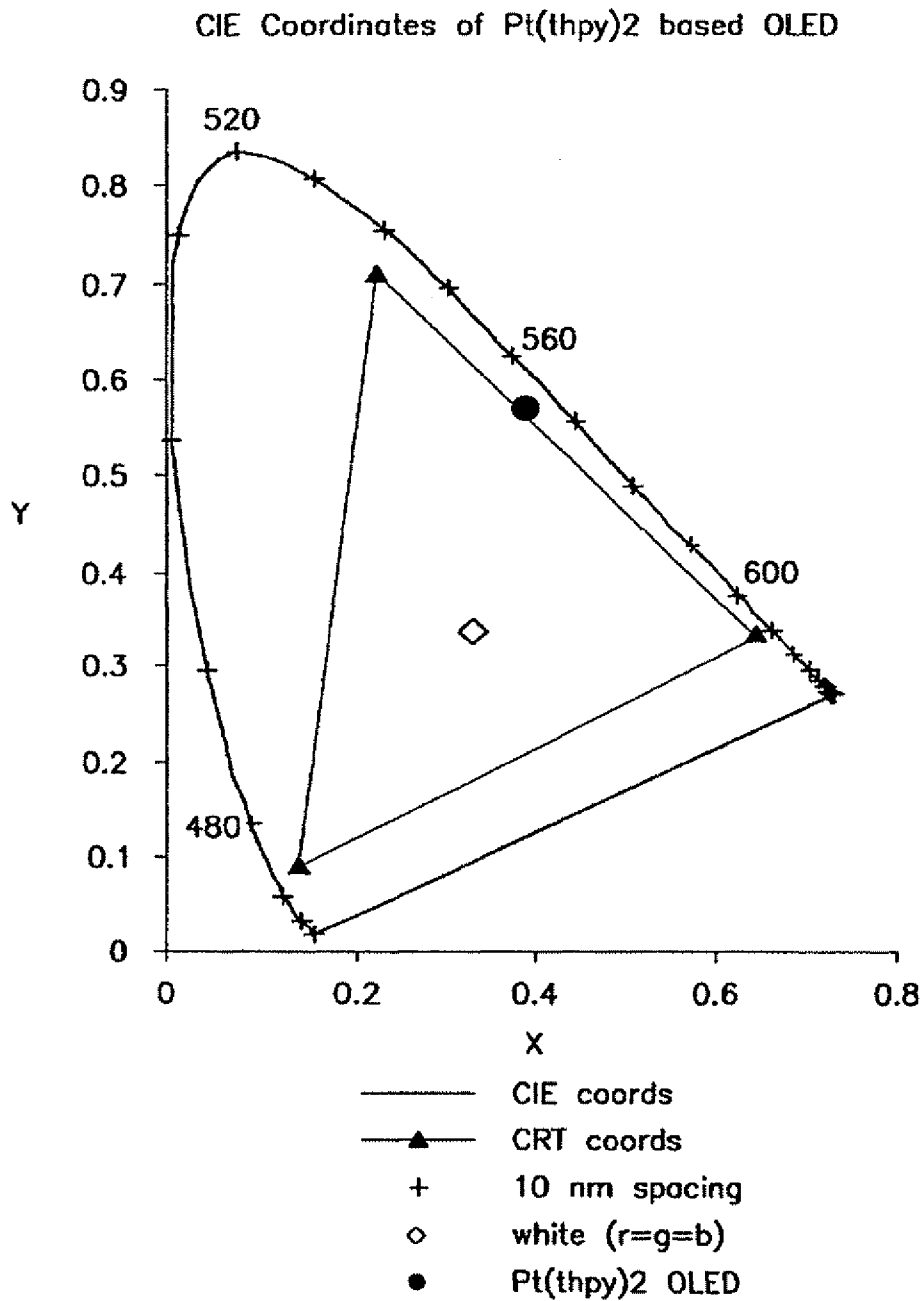
CIE diagram based on normalized EL spectrum
