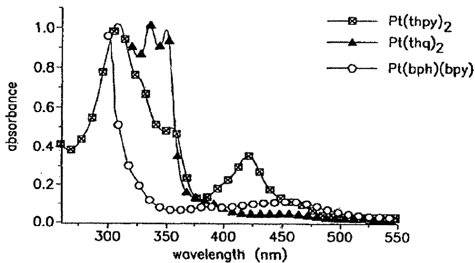
Electronic absorbance spectra of Pt(thpy) 2 , Pt(thq) 2 , Pt(bph)(bpy).
