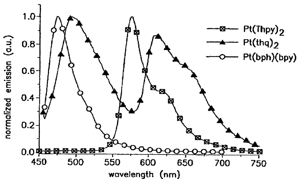
Emission spectra of the complexes.
