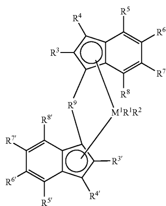
rac/pseudoracemic isomer
