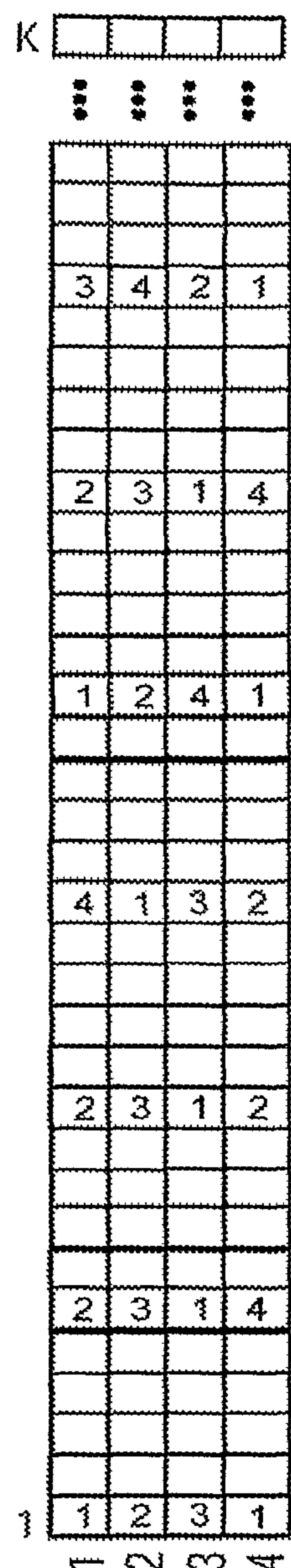
OFDM SYMBOL FOUR LAYER TRANSMISSION
