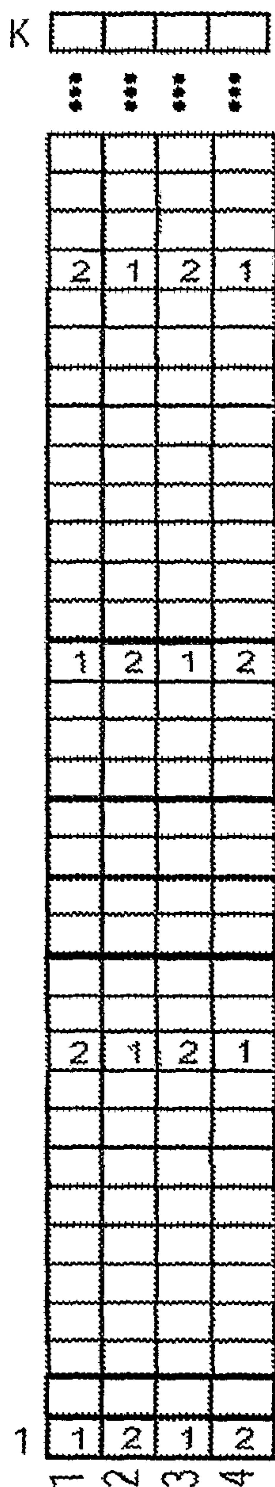
OFDM SYMBOL TWO LAYER TRANSMISSION
