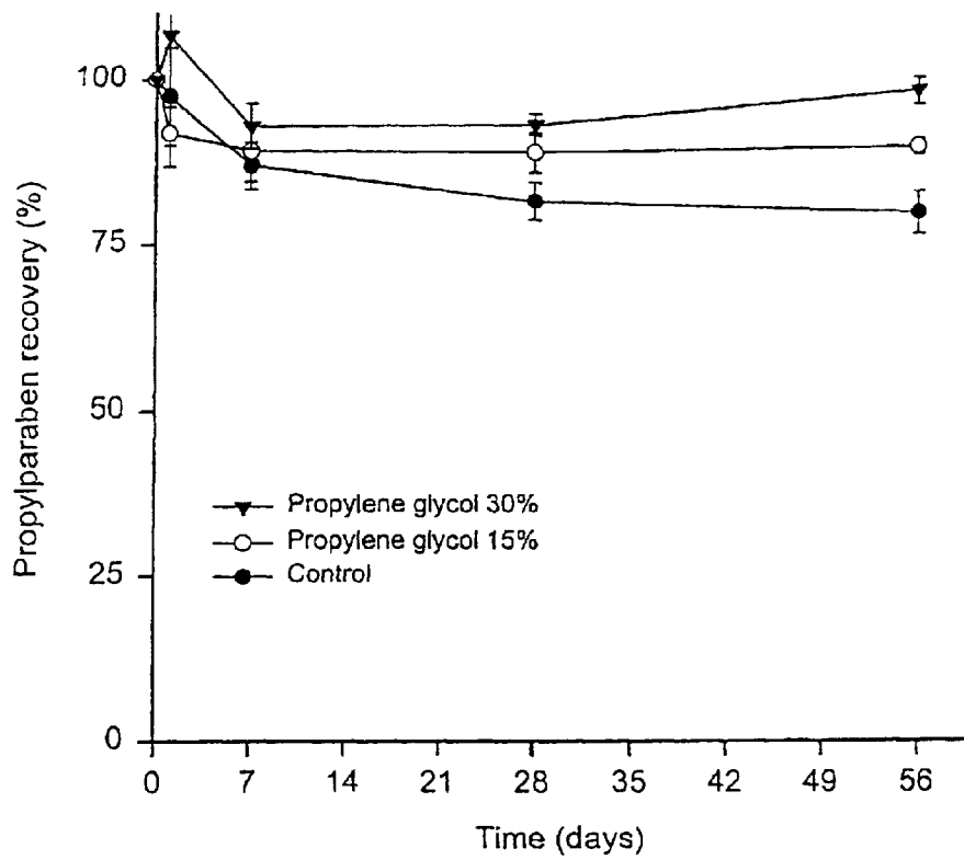
Effect of Propylene Glycol on Propylparaben Recovery Following Incubation with PETG
