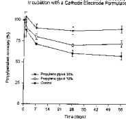
Effect of Propylene Glycol on Propylparaben Recovery Following Irradiation with a Cathode Electrode Formulation*
