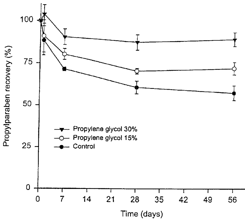
Effect of Propylene Glycol on Propylparaben Recovery Following Incubation with a Cathode Electrode Formulation*
