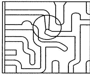
OPENS (NECKING) 33
