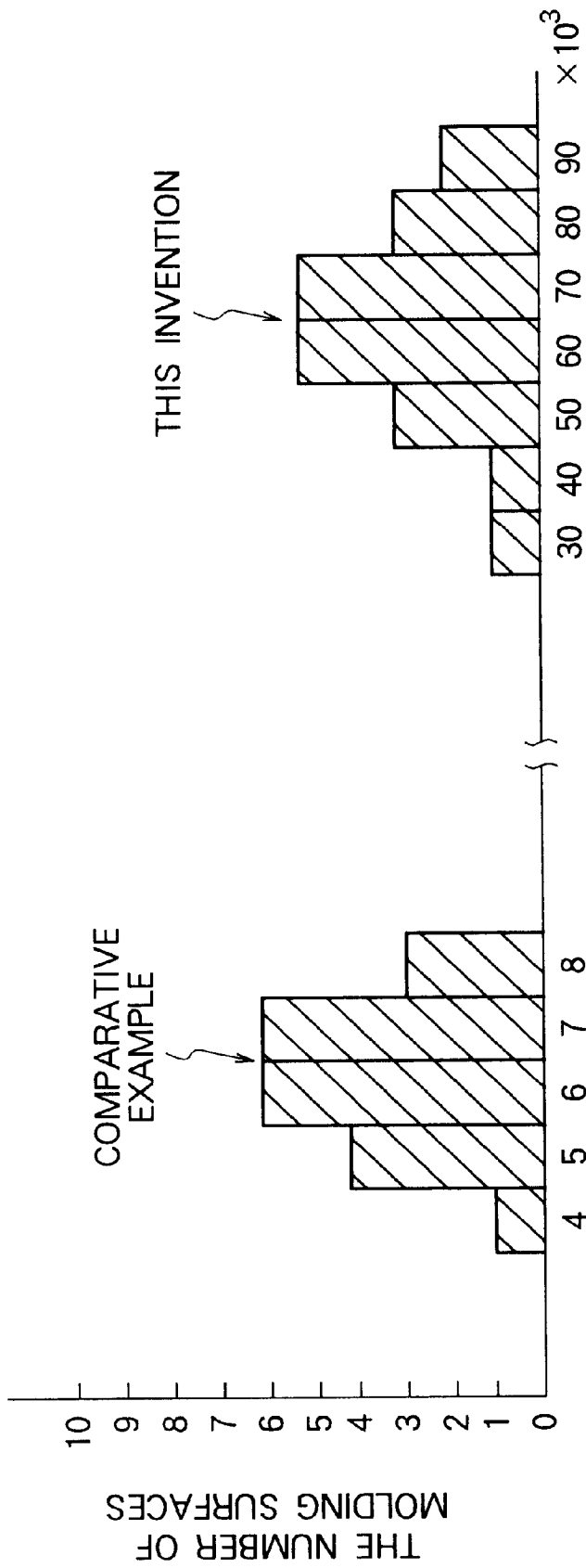
THE NUMBER OF TIMES OF PRESS-FORMING BEFORE THE MOLD CAN NOT BE USED DUE TO PULLOUT
