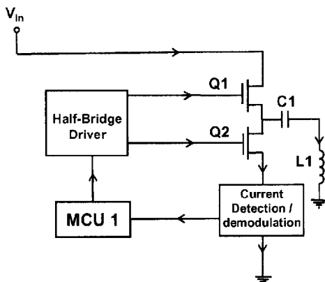
Charger
