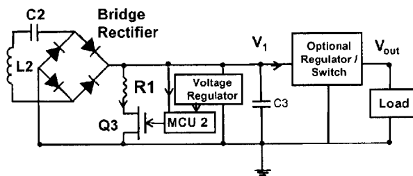
Receiver
