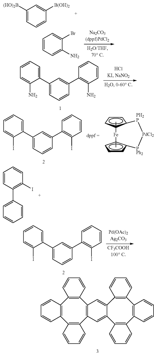
Scheme 1 Synthesis of Compound 3
