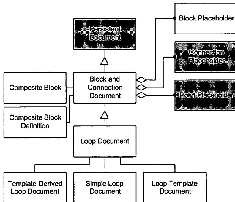
Figure 93 - Persistent Document Object derivations
