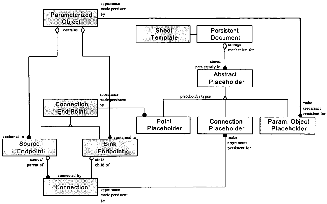
Figure 29A - Placeholders Object Model
