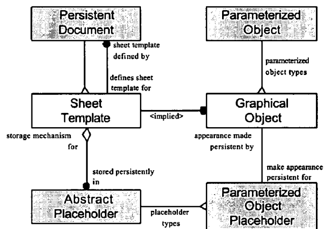
Figure 36 - Sheet Templates Object Model
