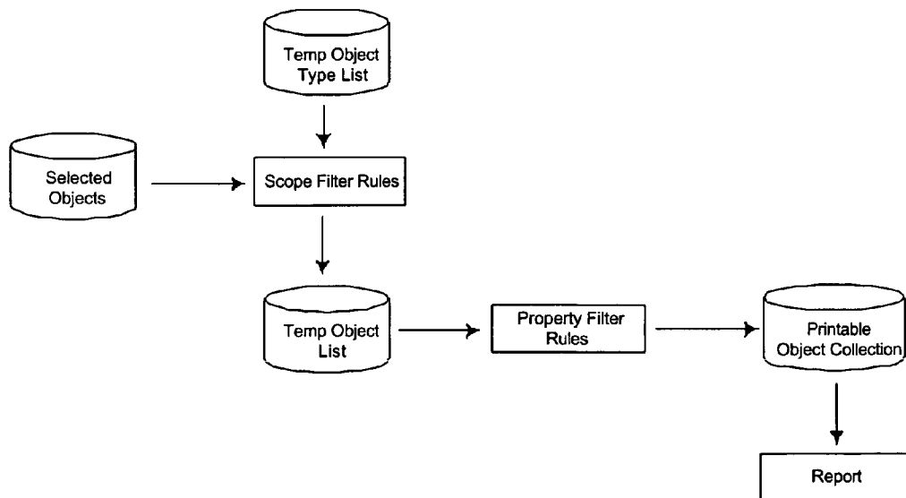
Figure 40 - Applying Filter Rules to POC
