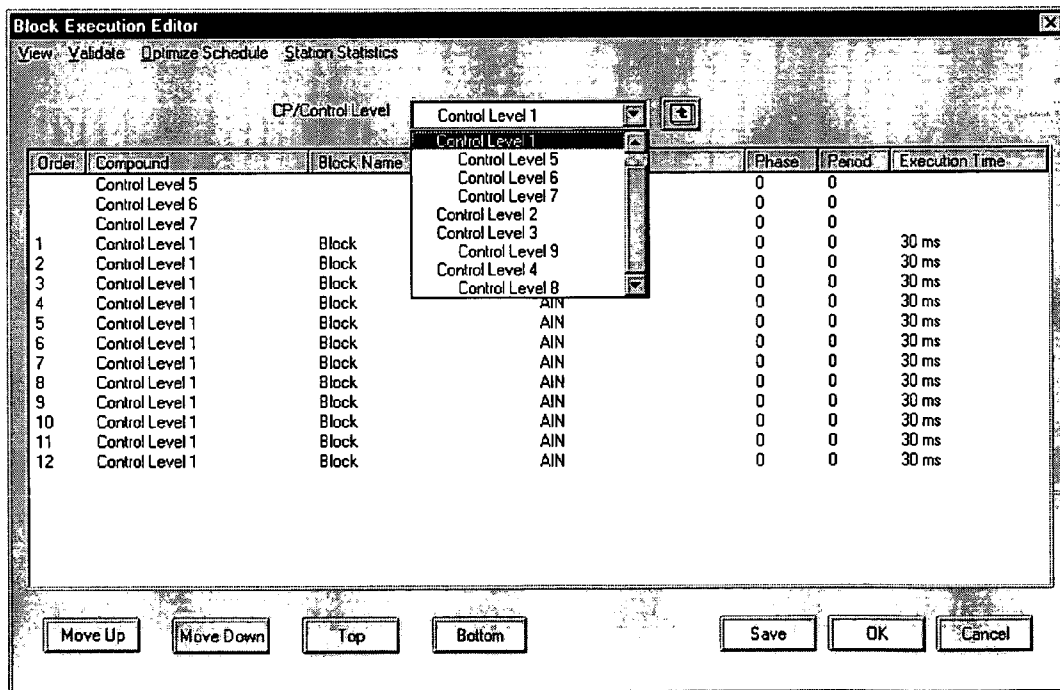
Figure 99 - Block Execution Scheduler Editor
