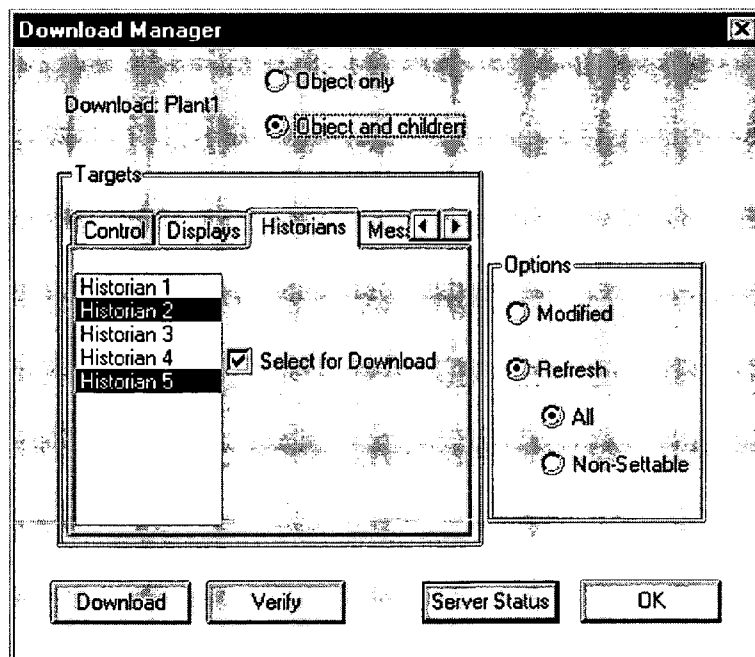
Figure 107 - Download Target Selection
