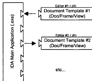
Figure 119 - IDA Main Application Architecture
