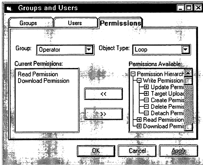
Figure 65 - Groups, Object Types and Permissions
