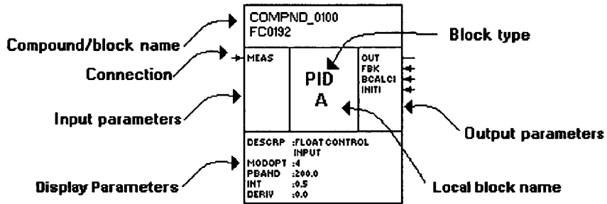
Figure 76 - Anatomy of a Block Placeholder
