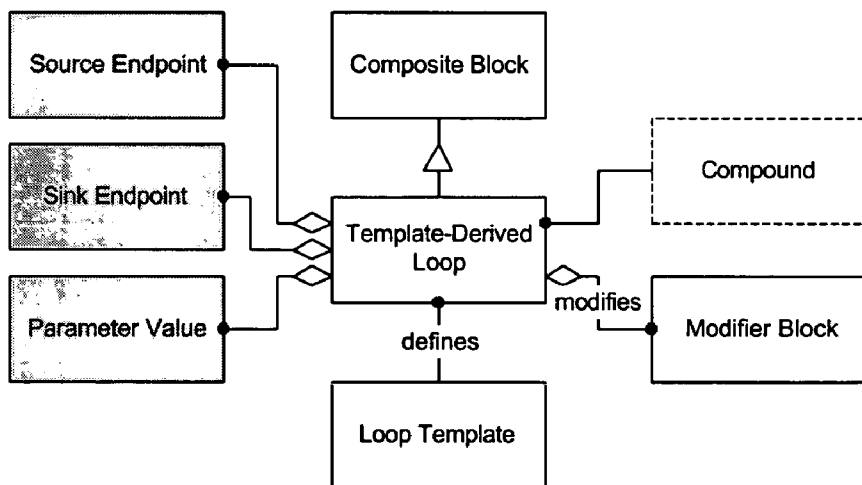
Figure 91 - Template-Derived Loop object model
