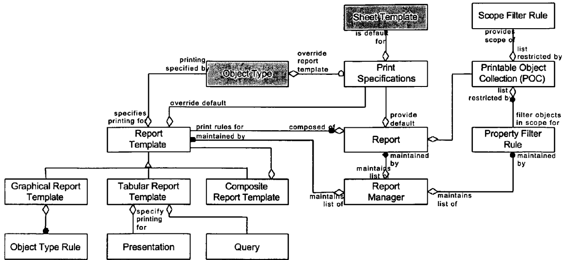
Figure 39 - The IDA Report Manager Object Model
