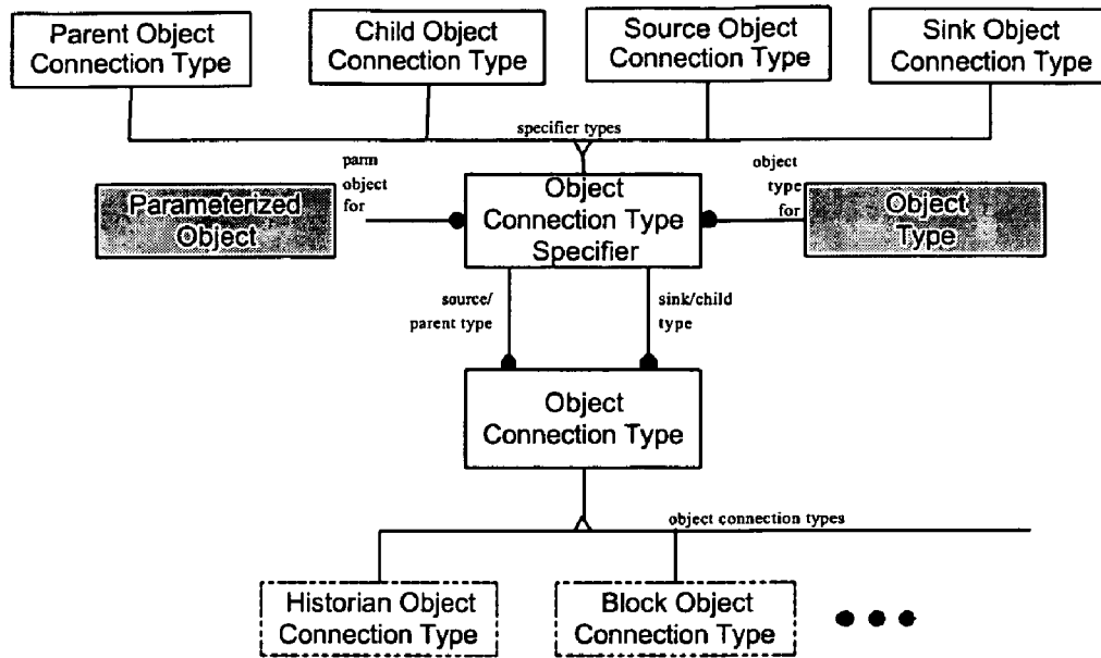
Figure 19 - Object Connection Type Object Model
