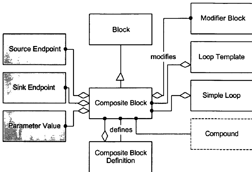
Figure 90 - Composite Block object model
