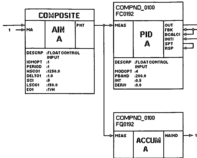
Figure 73 - Composite Block In Loop
