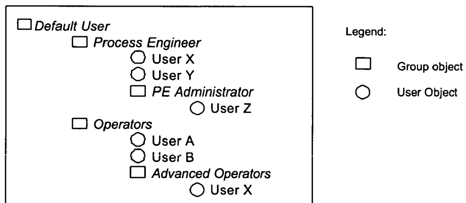
Figure 59 - Users and Groups Example
