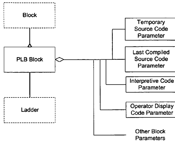
Figure 98 - PLB Block Model
