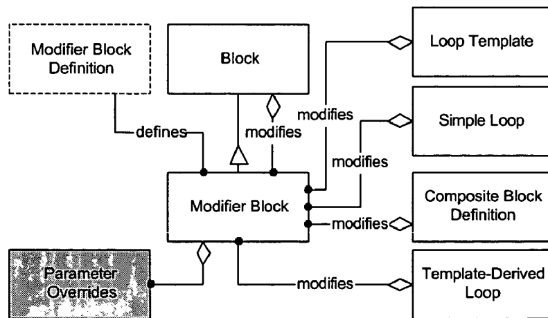
Figure 85 - Modifier Block object model
