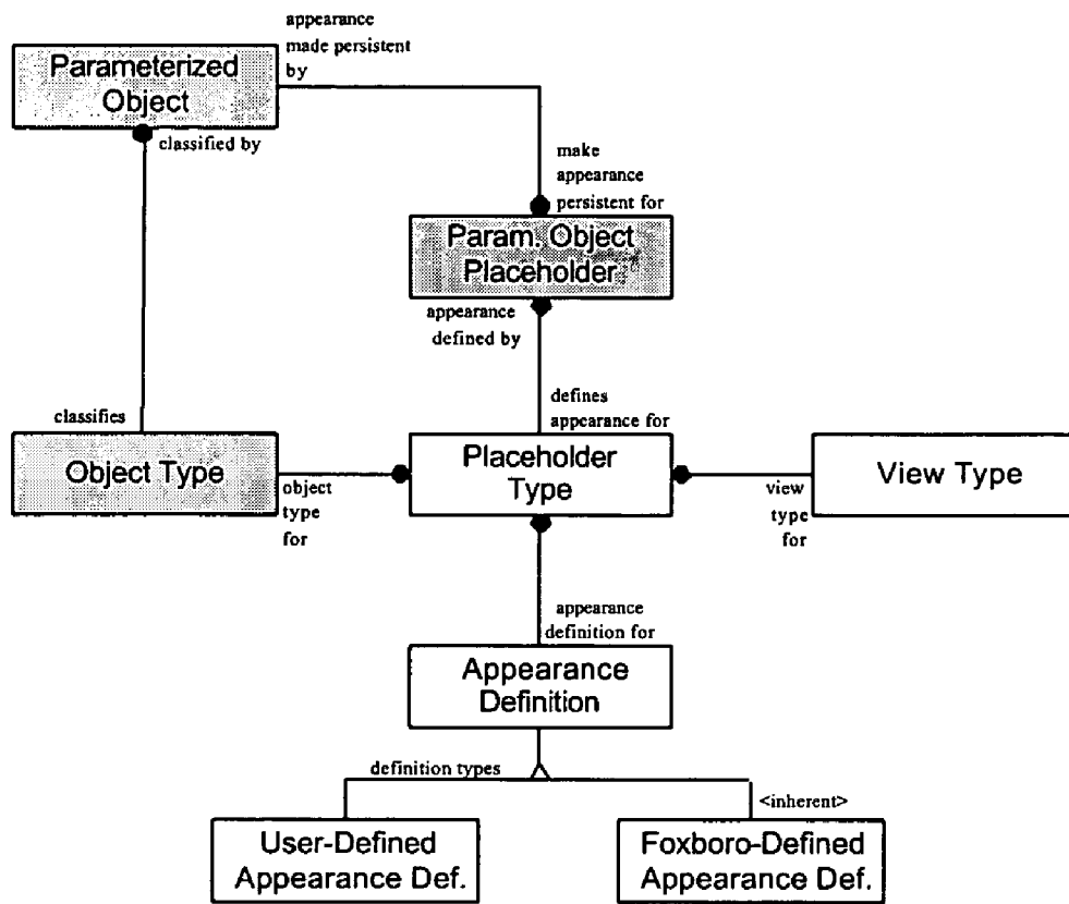
Figure 27 - Appearance Object Model
