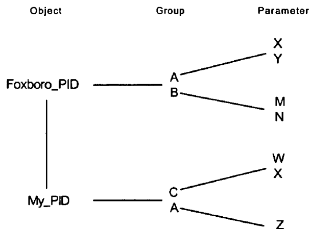
Figure 8 - Parameter Group Inheritance
