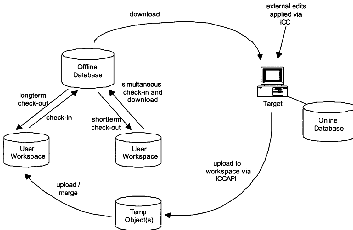
Figure 45 - Version Control - Basic Concepts
