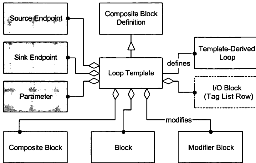
Figure 88 - Loop Template object model
