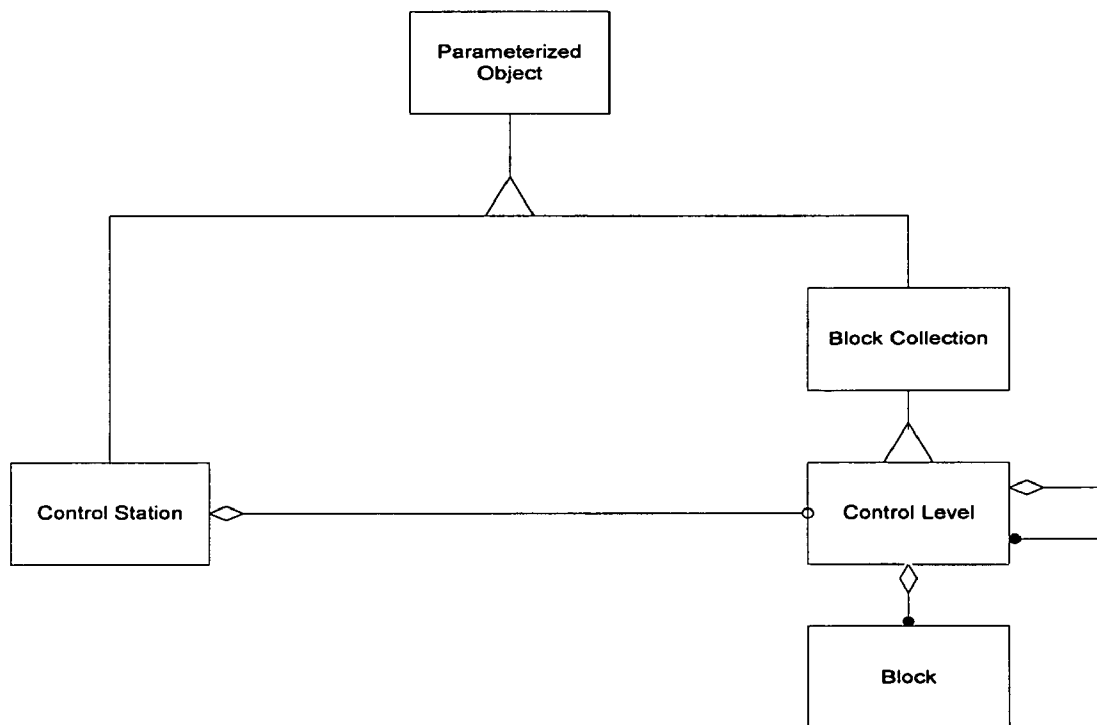
Figure 101 - Block Execution Editor Object Model
