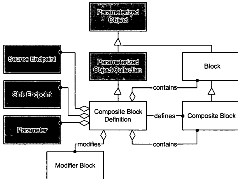
Figure 87 - Composite Block Definition object model
