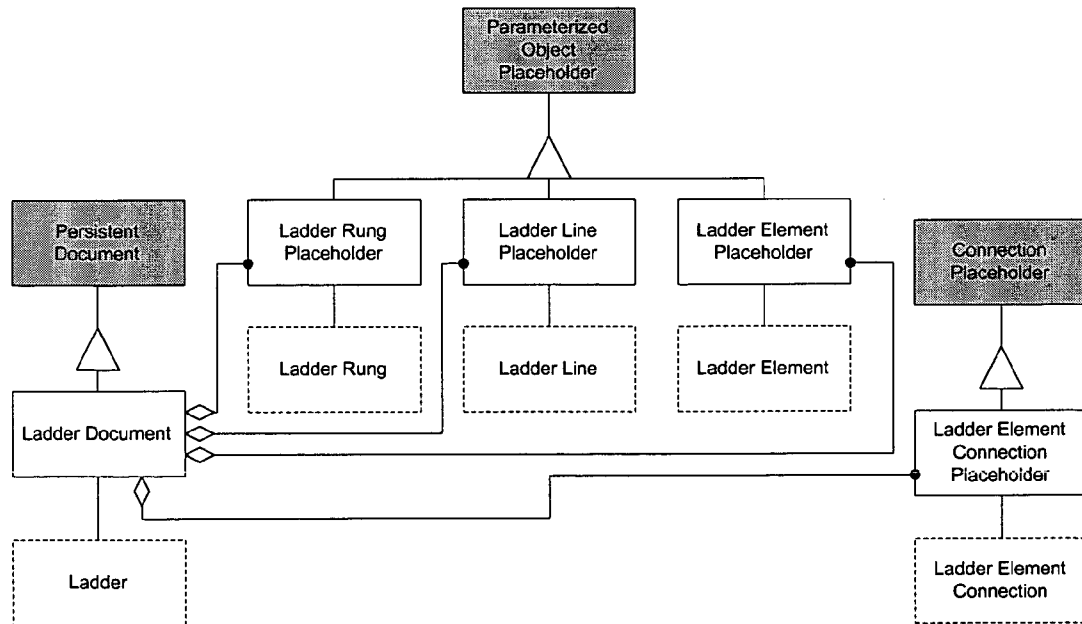
Figure 97 - Persistent Document Objects.
