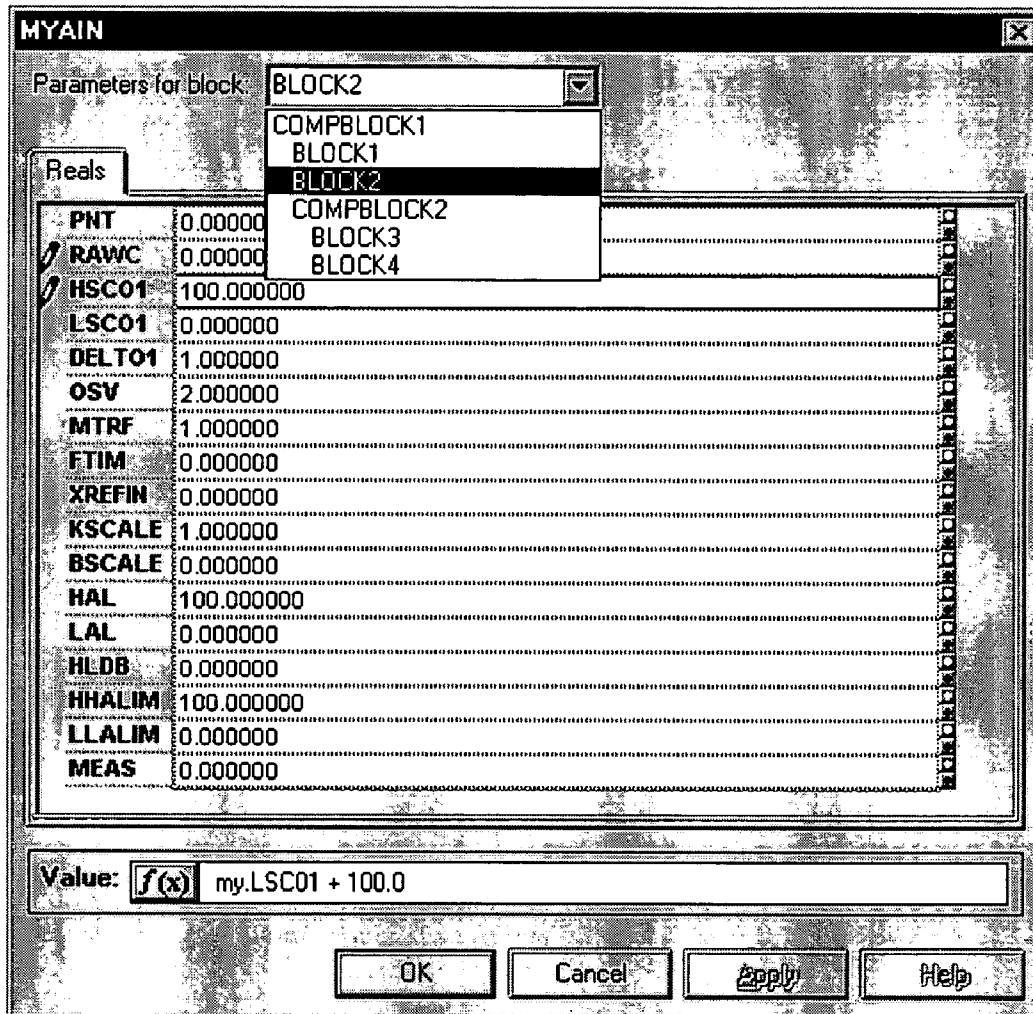
Figure 81 - Composite Block Property Sheet
