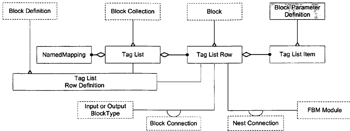
Figure 106 - Tag List Object Model
