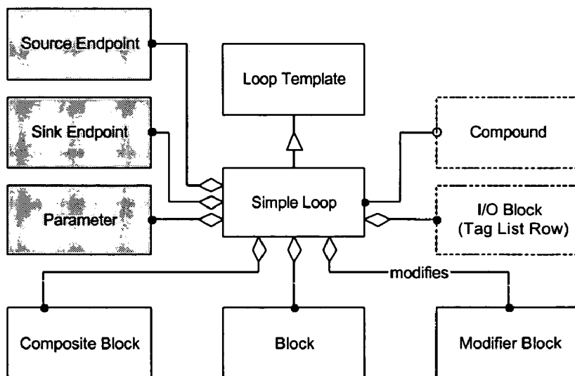
Figure 89 - Simple Loop object model
