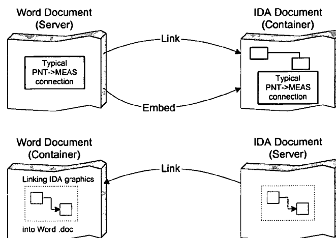
Figure 121 - IDA & OLE Compound Documents
