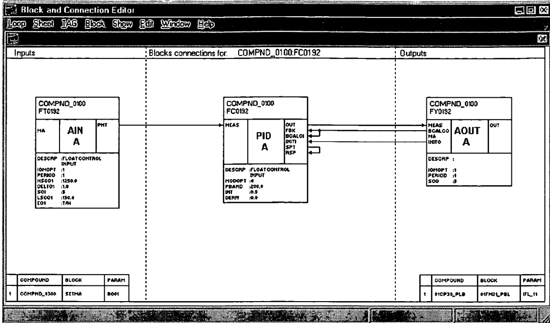
Figure 75 - Block with Connections
