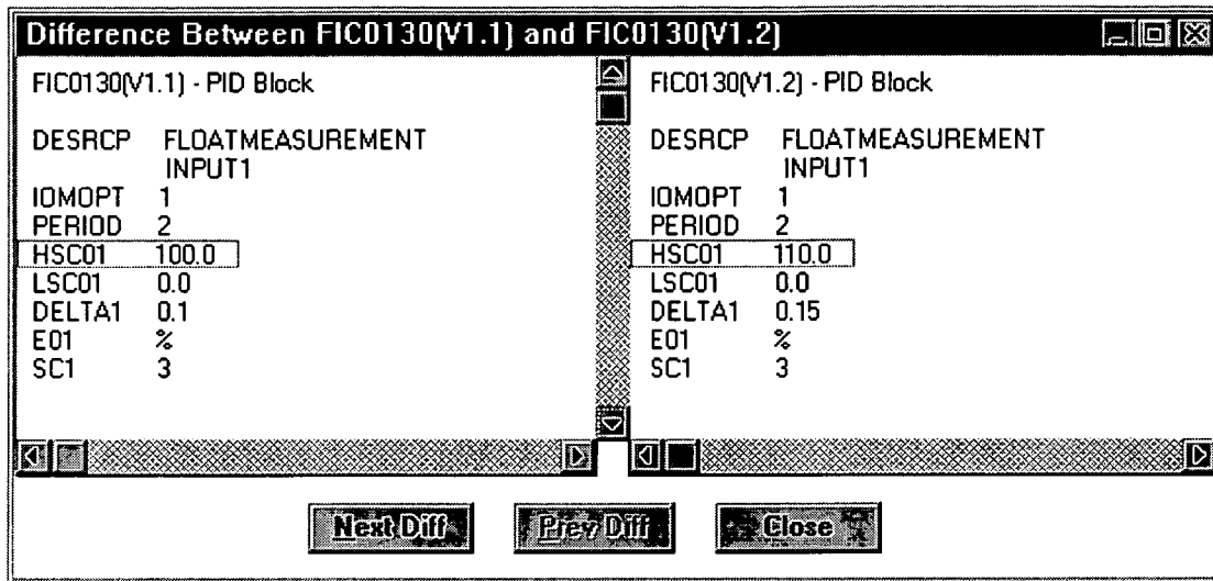
Figure 53 - Object Compare Utility
