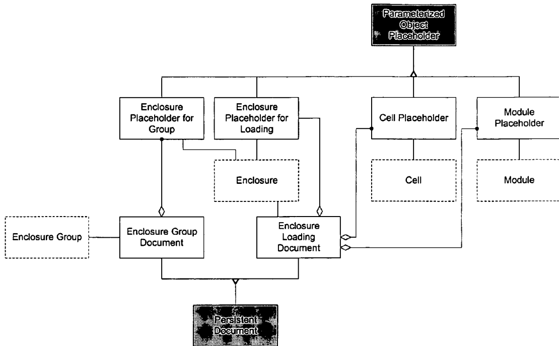
Figure 118 - Persistent Document Objects.
