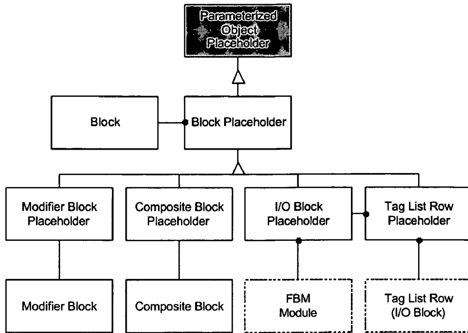
Figure 92 - Object Placeholder derivations
