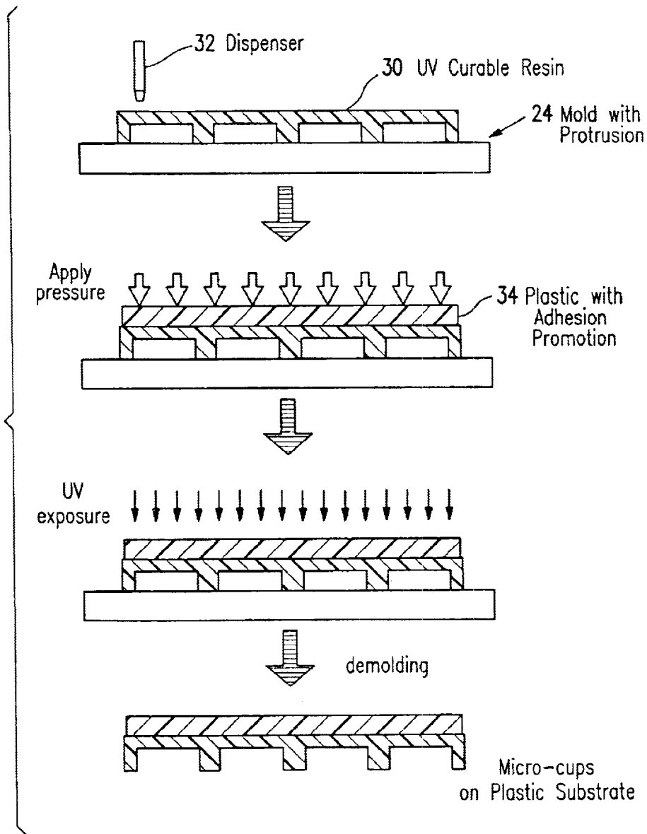
Transfer Molding with Resin Dispensed on Mold
