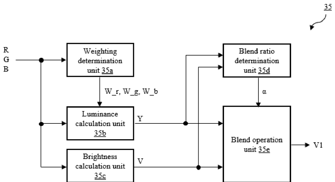
FIG. 8 Second embodiment
