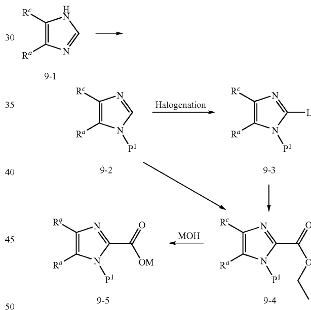
Scheme 9
