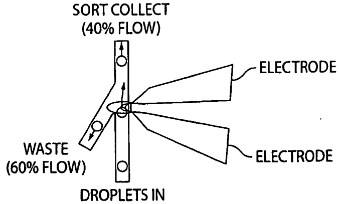
INVERTED FLUIDIC GEOMETRY (ASYMMETRIC FLOW GEOMETRY)
