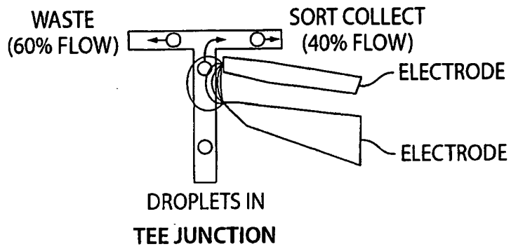
TEE JUNCTION
