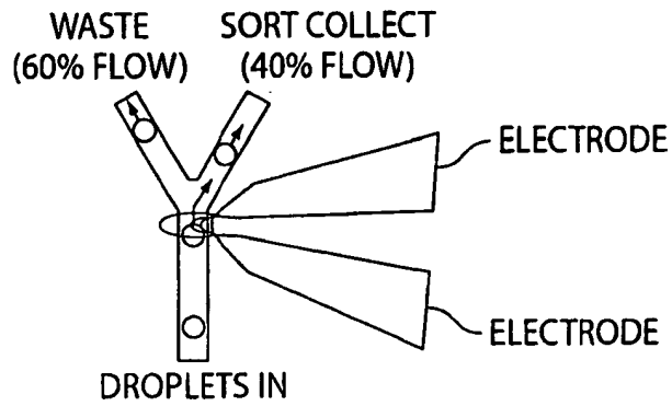
DESIGN IMPLEMENTED
