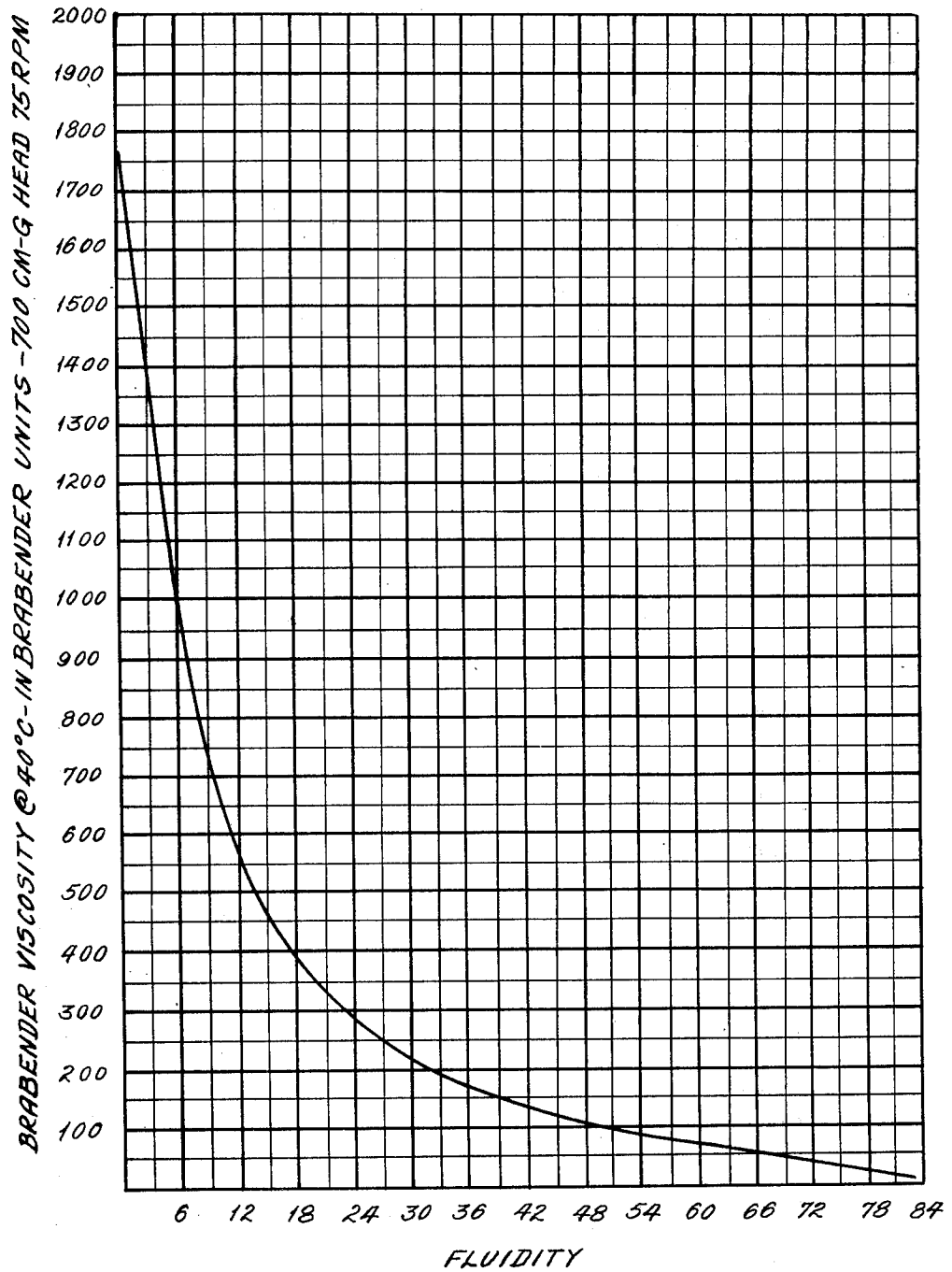
BRABENDER VISCOSITY @ 40°C VS. FLUIDITY
